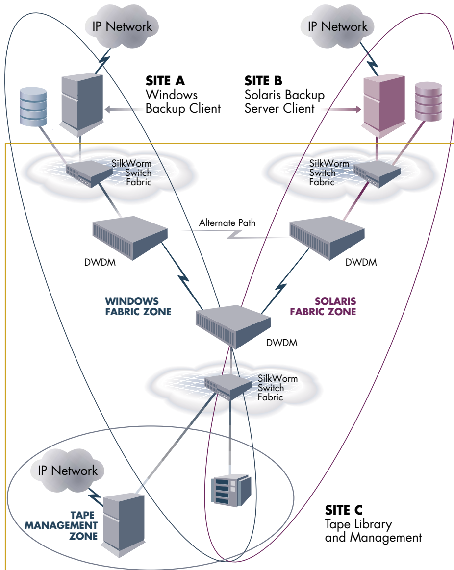
Figure 14. Centralized remote backup over a MAN
