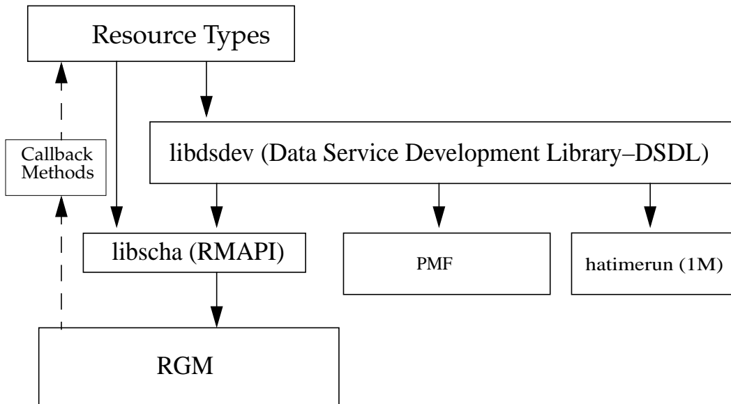
FIGURE 1-1 Programming Architecture
