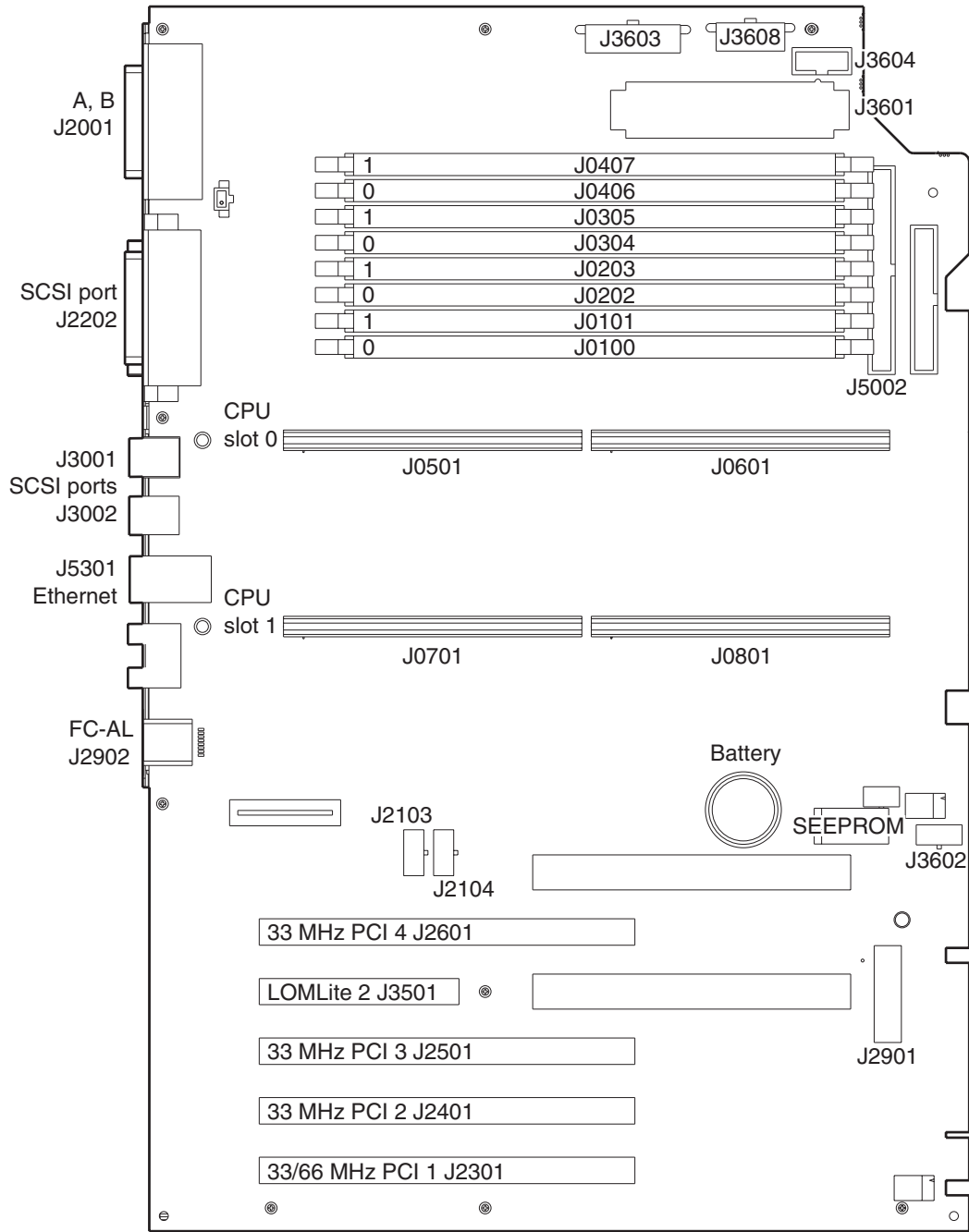
FIGURE 2 Netra 20 Server System Board
