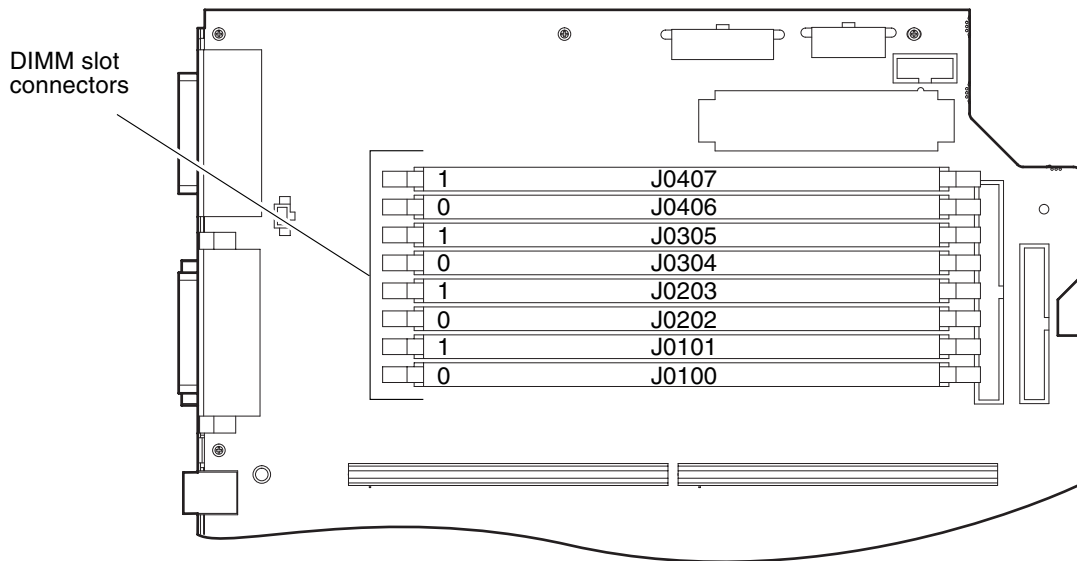
FIGURE 1 Netra 20 Server DIMM Slot Connectors With Correct Reference Designators
