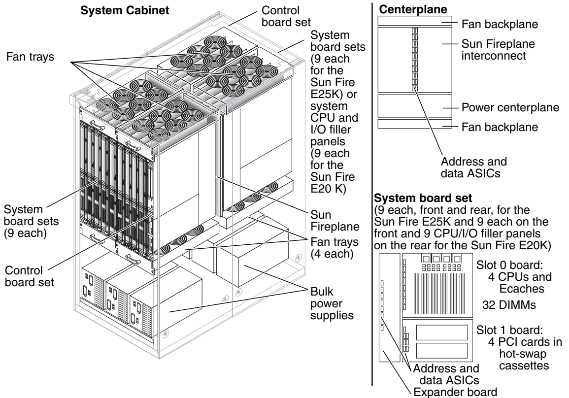
FIGURE 5-1 Sun Fire E25K/E20K Systems Major Components
