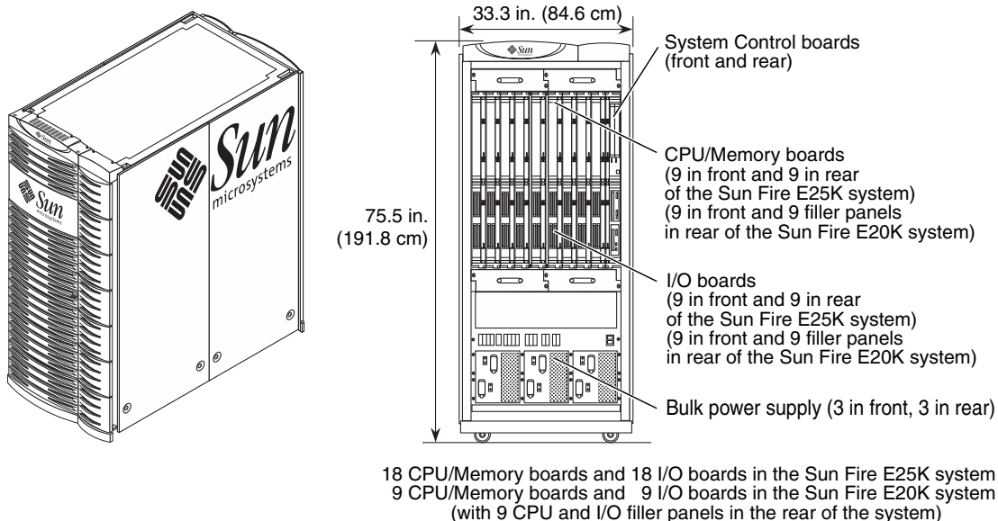
FIGURE 1-1 Sun Fire E25K/E20K Systems
