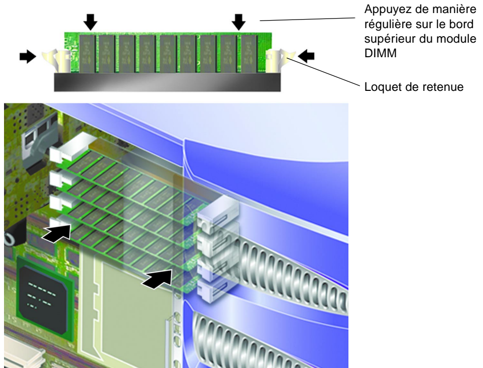
FIGURE 1-15 Insertion d'un DIMM
