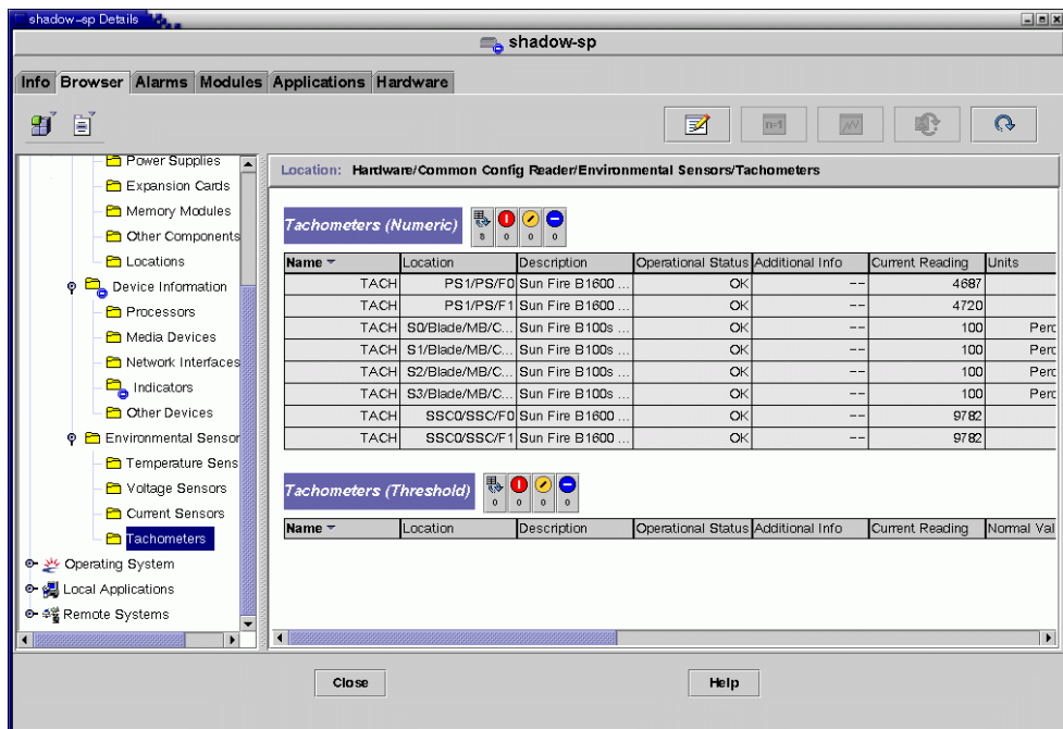
FIGURE 4-3 Part of the Tachometers Table
