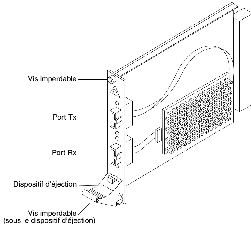
FIGURE 1-6 Module optique Sun Fire Link
