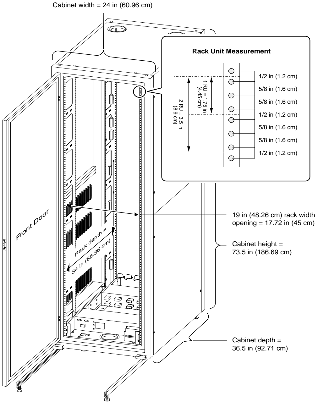
FIGURE 3-3 EIA 310D-Compliant Cabinet and Rack
