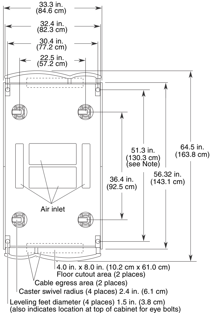
FIGURE 1-6 Sun Fire 15K/12K Systems Floor Cutout and Base Dimensions Diagram
