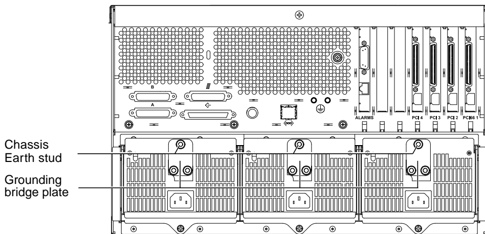
FIGURE 1 Grounding Points
