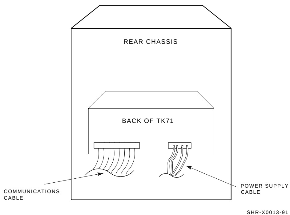
Figure 6-13 Cabling at Rear of Drive
