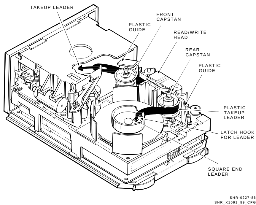
Figure 6-16 TK71 Tape Path (Takeup Leader Replaced)
