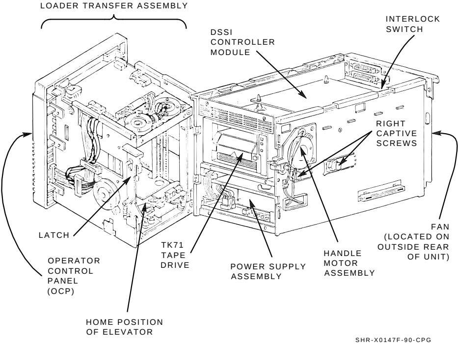
Figure 6-7 Loader Transfer Assembly Latch Position
