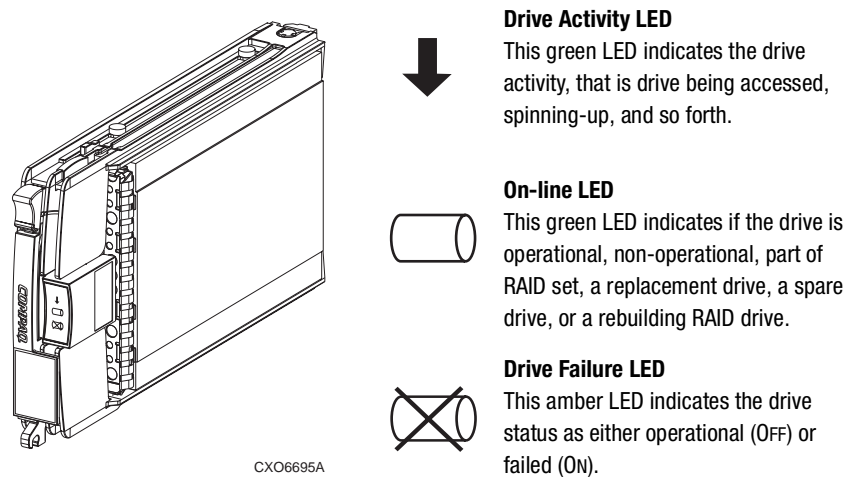
Figure 4-2. Disk Drive LEDs Display
