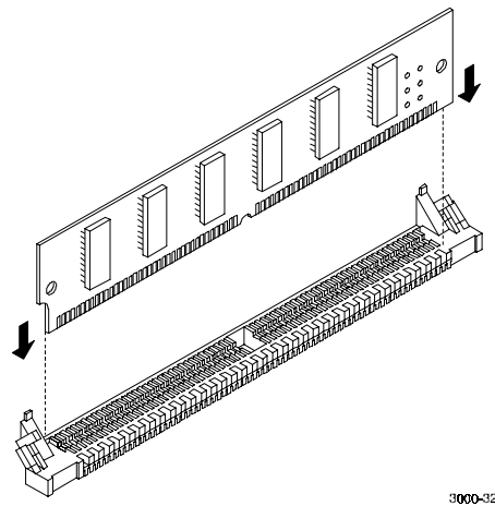
Figure 4–5 Insert Module into SIMM Connector
