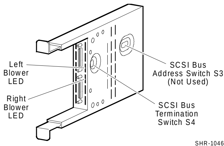
Figure 1-6 Device I/O Module Blower Status LEDs
