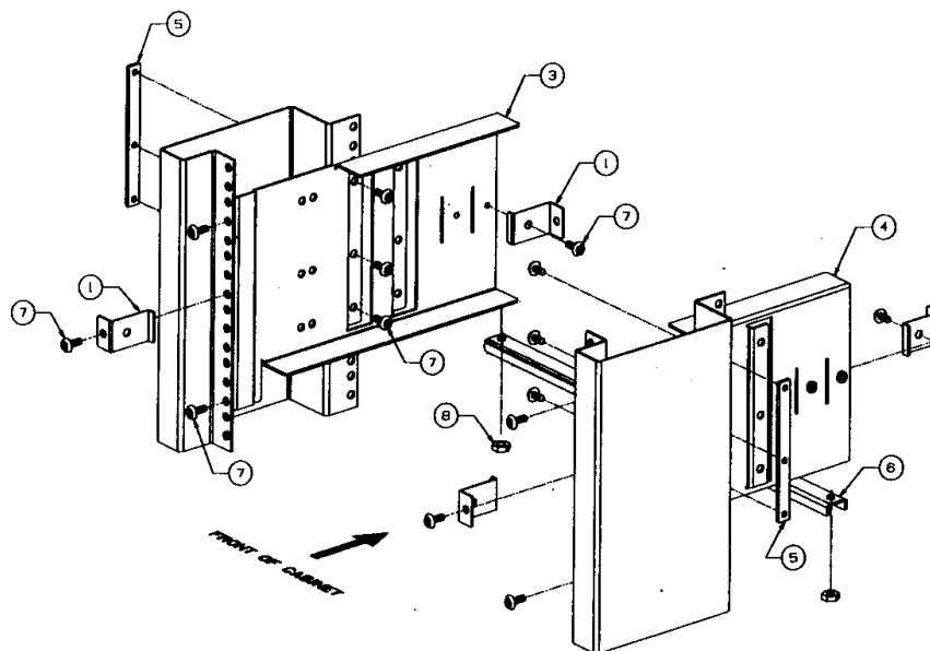
Figure 3–5 RETMA Cabinet Shelf Supports
