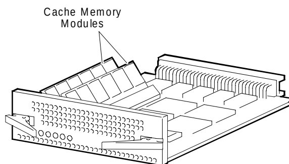
Figure 3–20 Release Locking Clips
