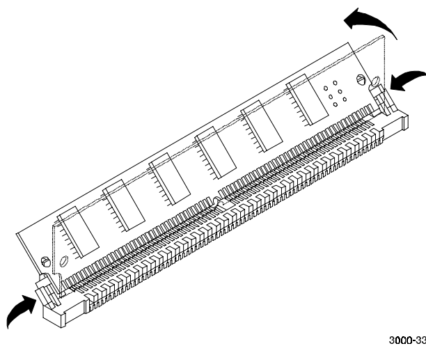
Figure 3-23 Pivot Module Down to Secure
