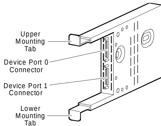
Figure 1–5 Device I/O Module
