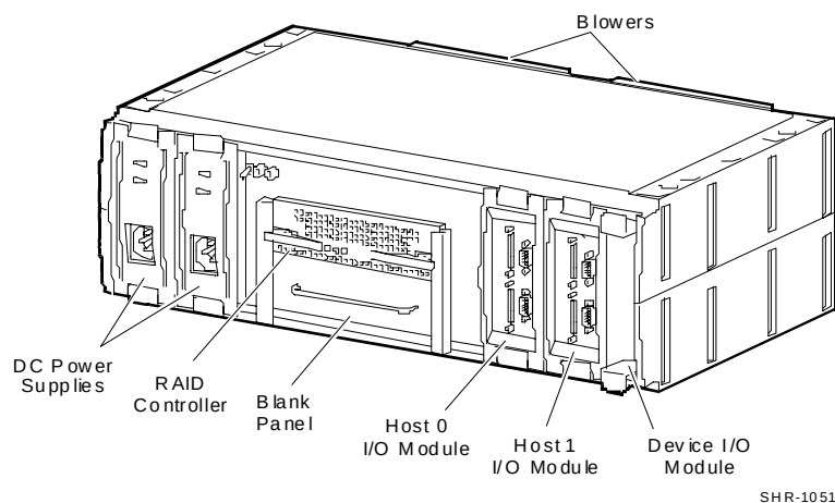
Figure 1–3 Controller Shelf Major Components
