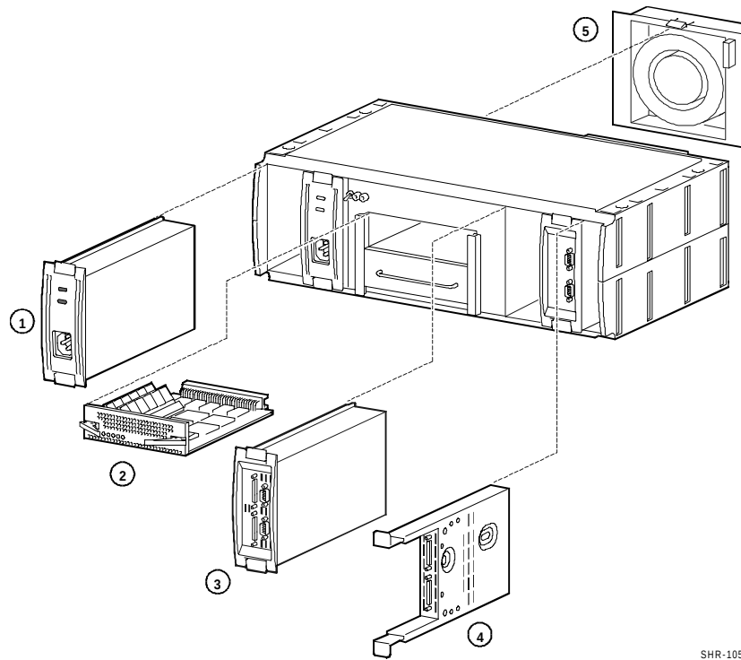
Figure 3–15 Controller Shelf Field Replaceable Units
