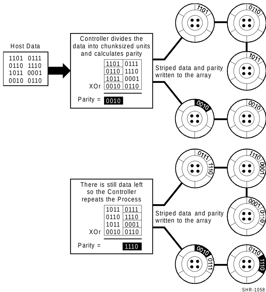
Figure 2–9 Diagram of a RAID 5 Write
