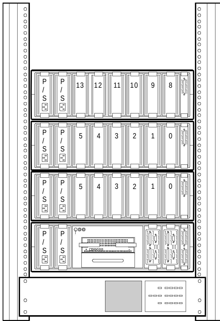
Figure 3-3 Recommended Controller Shelf Installation (Three Expansion Shelves)
