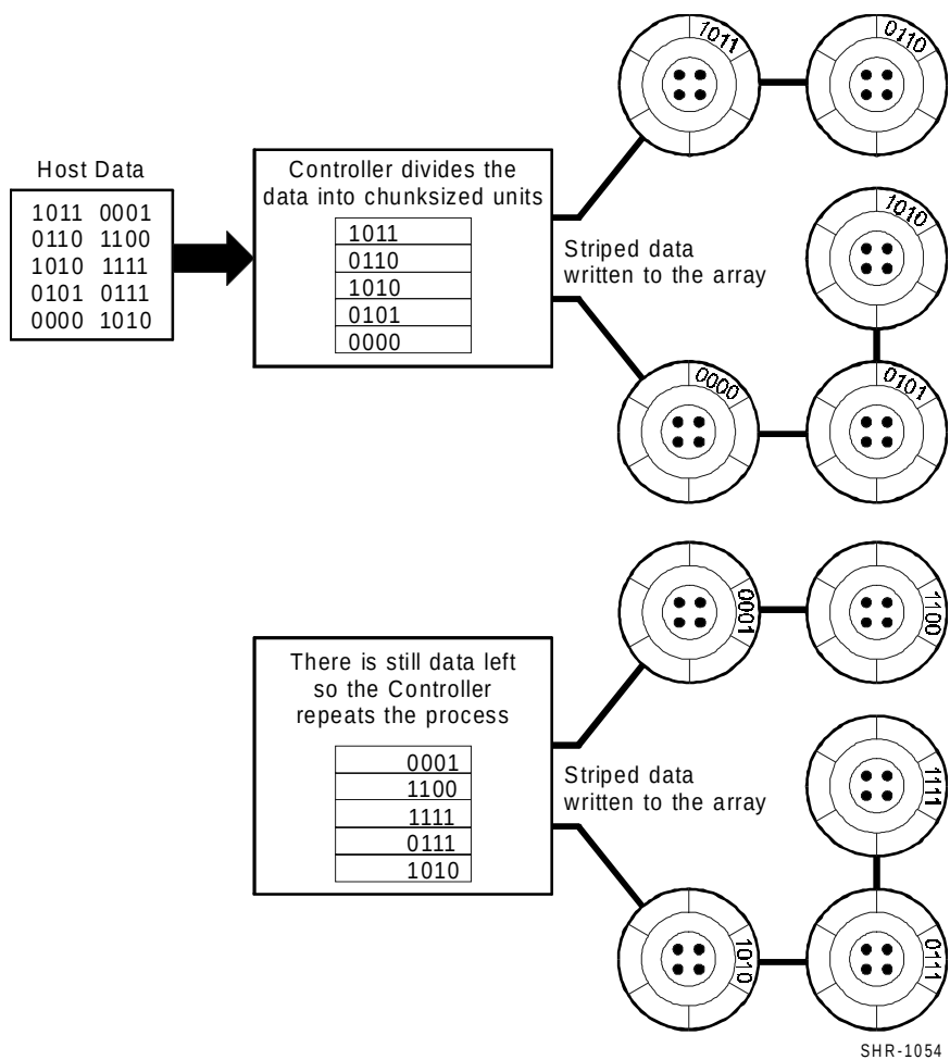
Figure 2-5 RAID 0 Write
