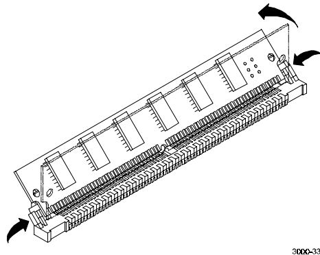
Figure 4–6 Pivot Module Down to Seat
