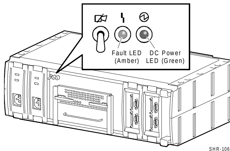
Figure 3–14 Shelf Status LEDs
