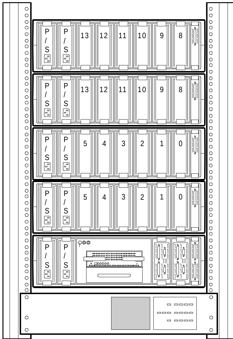
Figure 3-4 Recommended Installation (Four Expansion Shelves)
