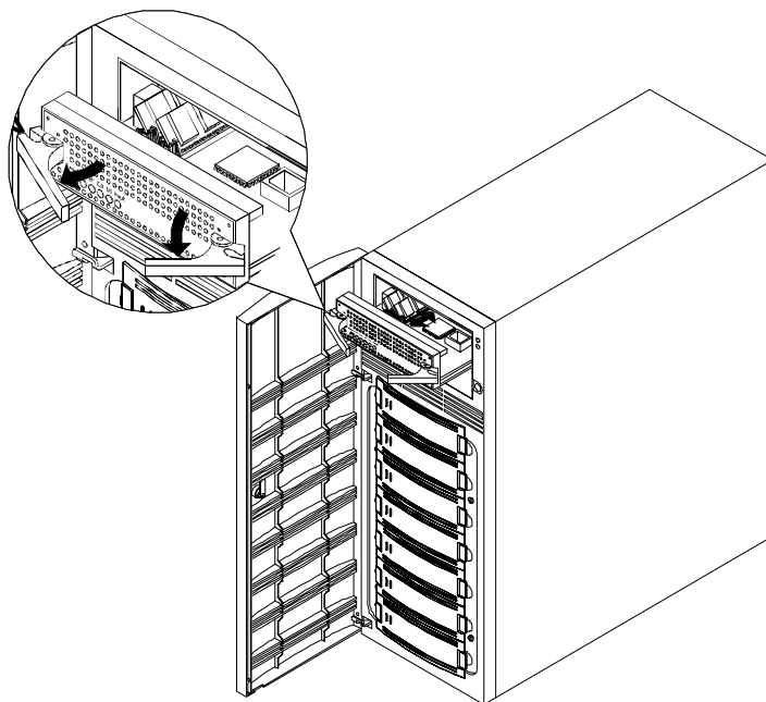
Figure 5-8. Remove Controller from Top Slot
