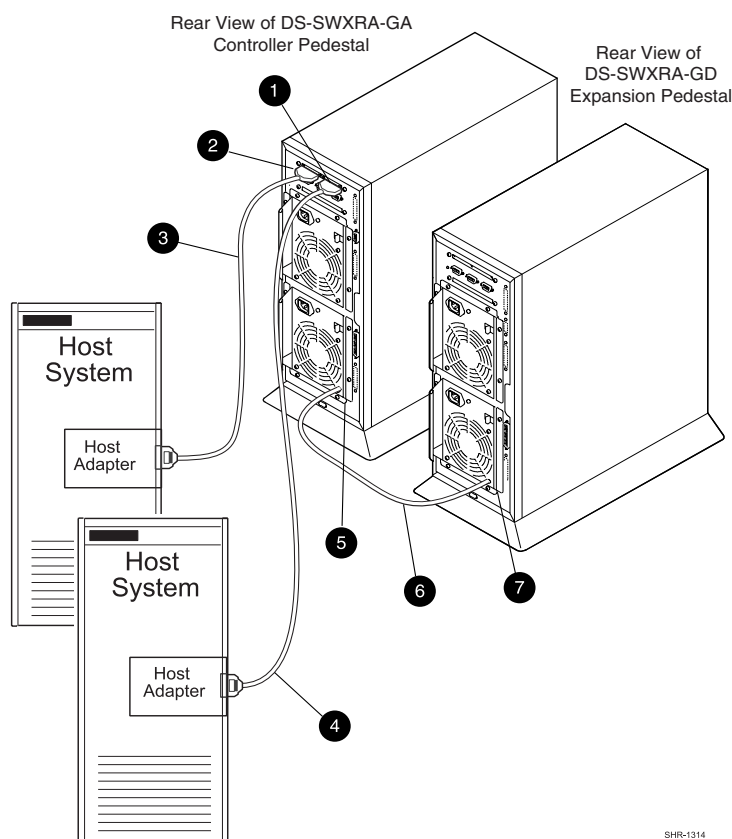
Figure 1–12 Dual Host, Single Adapter/Single Controller Cabling Diagram
