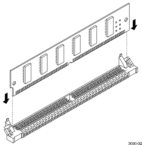
Figure 5-6. Insert Module into SIMM Connector
