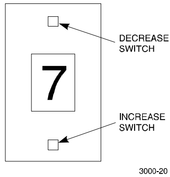
Figure 4-13 Reconfigured SCSI Bus Addresses
