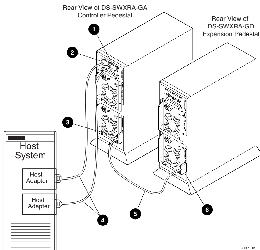
Figure 1–10 Single Host, Dual Adapter/Dual Controller Cabling Diagram
