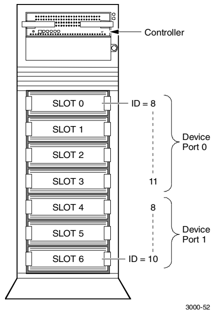
Figure 1-8 Slot Locations and SCSI ID Addresses
