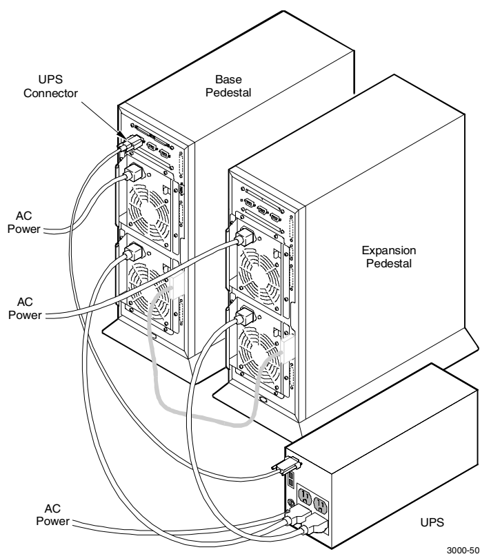
Figure 4–15 Power Cable Connections
