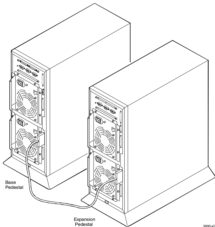
Figure 4-14 Connect SCSI Cable Between Pedestals
