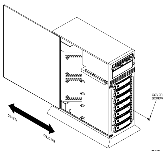
Figure 4-5 Remove Side Cover from Base Pedestal
