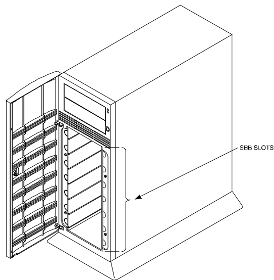
Figure 4-1 Expansion Pedestal
