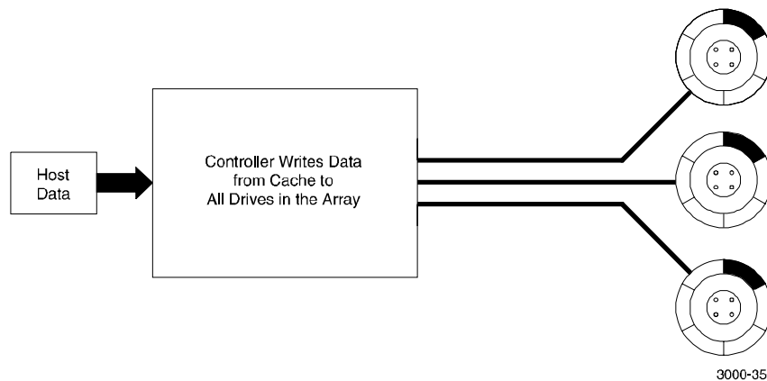
Figure 2–5 Diagram of a RAID 1 Write
