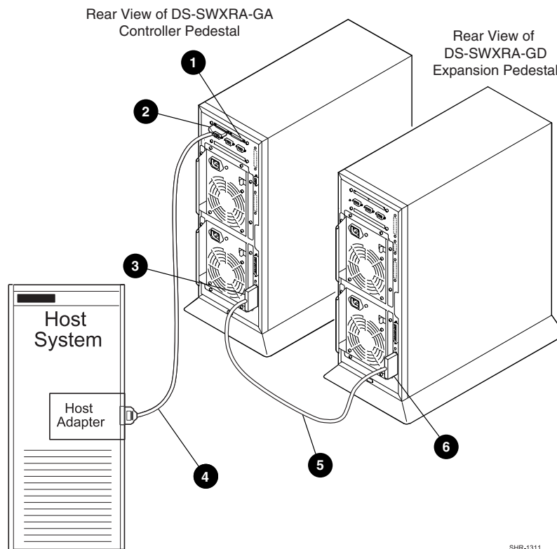
Figure 1–9 Single Host, Single Adapter Cabling Diagram
