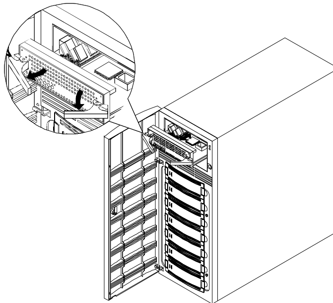
Figure 3–6 Removing the Controller from the Pedestal
