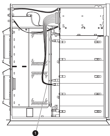
Figure 4-7 Disconnect SCSI Cable
