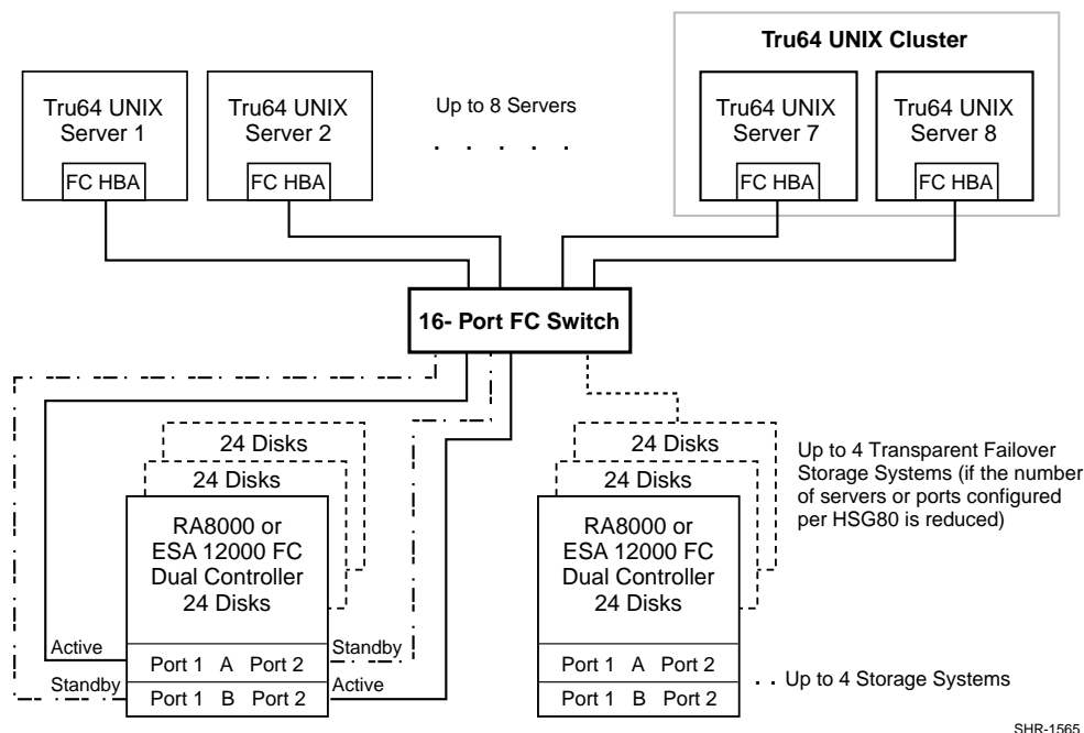
Figure 1 SAN Configuration
