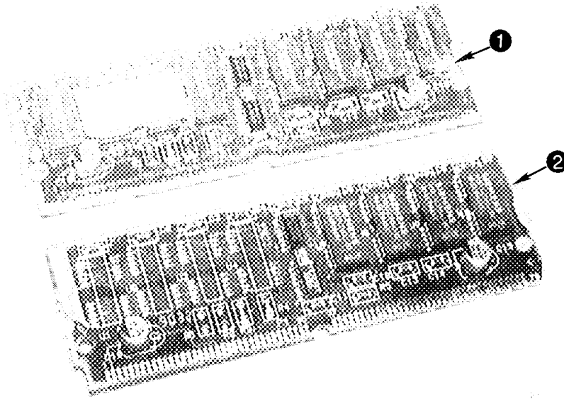
Figure 9-1 Memory SIMs
