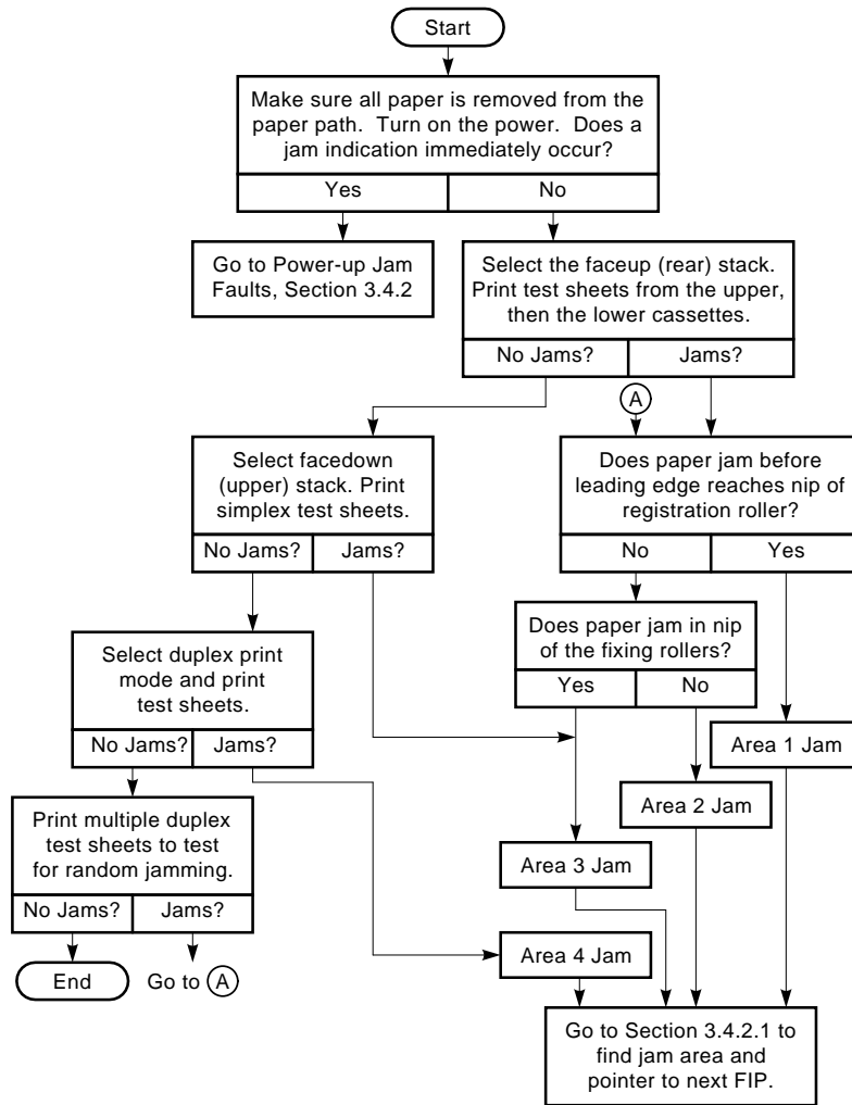
Figure 3–3: Jam Start FIP
