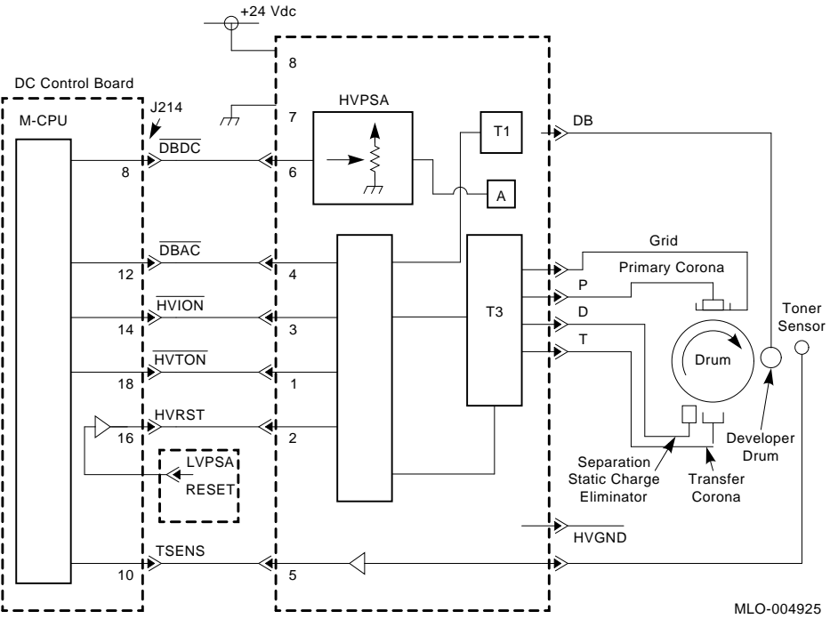
Figure 1-19: HVPSA Image Circuits
