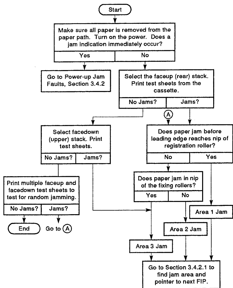
Figure 3-3: Jam Start FIP
