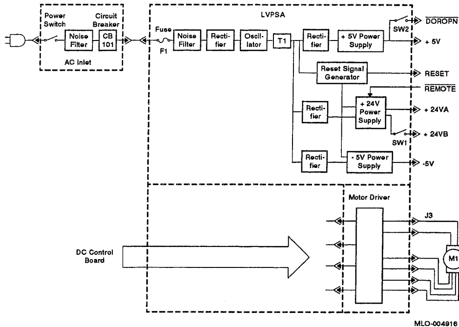
Figure 1–12: LVPSA Block Diagram
