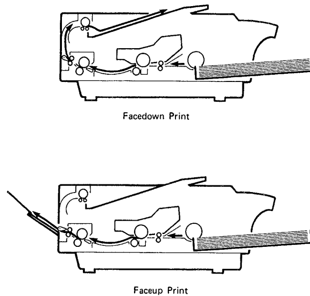
Figure 1-6: 2100 Paper Paths
