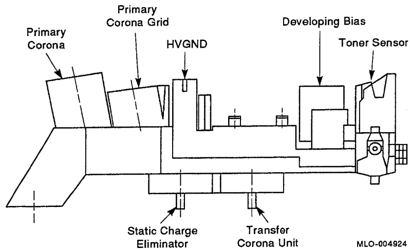
Figure 1-14: HVPSA Connector Block
