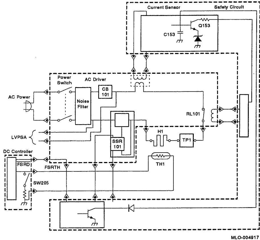
Figure 1–13: Fixing Heater Diagram
