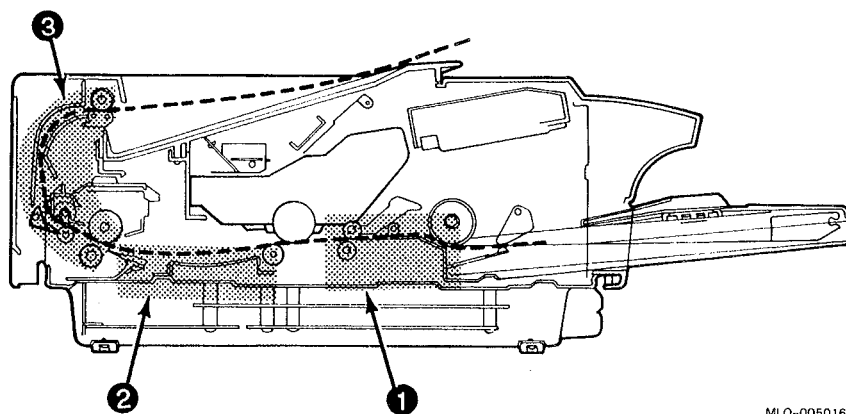
Figure 3-4: 2100 Jam Areas
