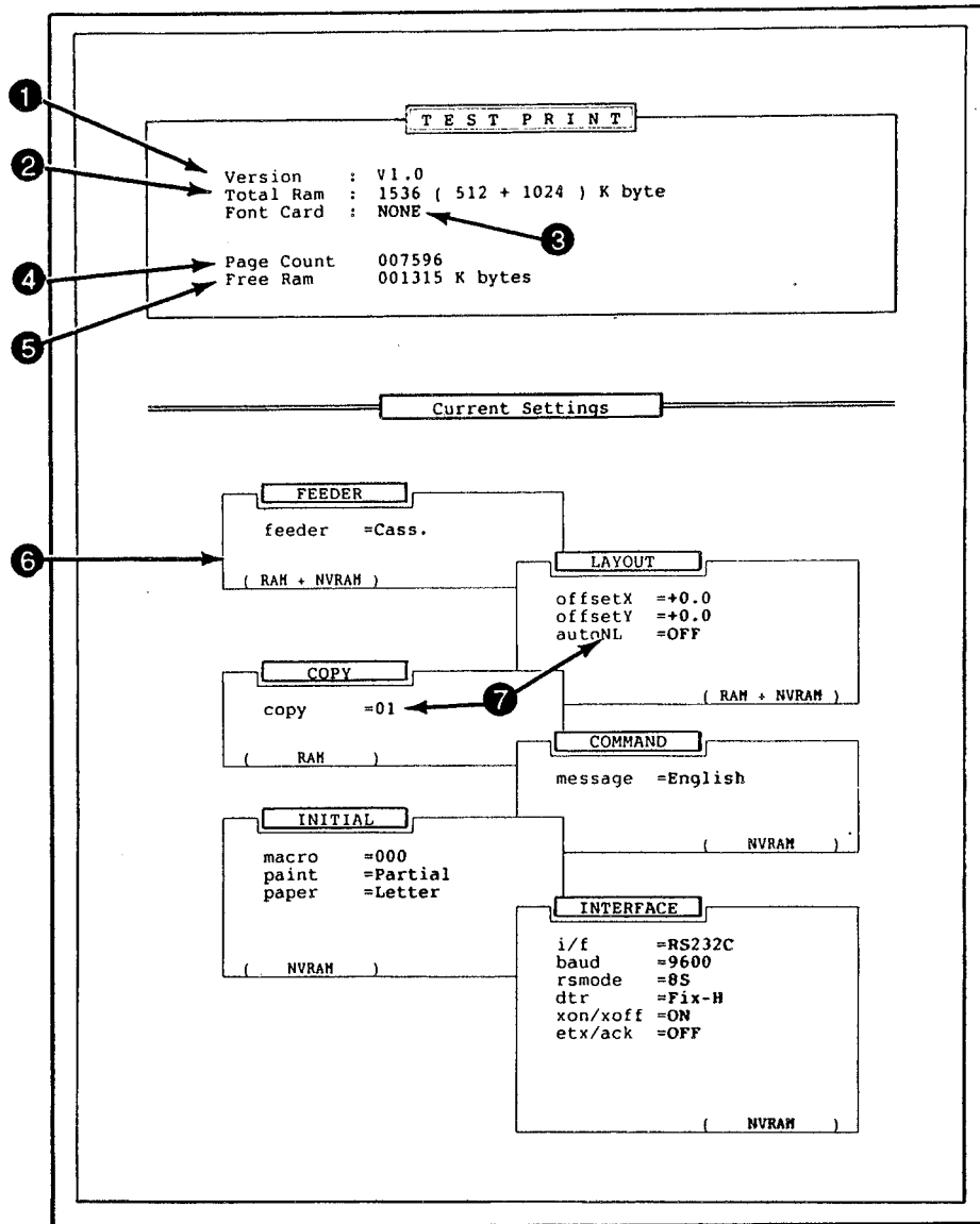
Figure 2-5: Test Print A
