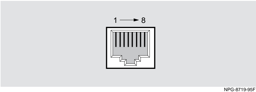
Figure B-1: 10BaseT (8-Pin MJ) Straight-Through Connector
