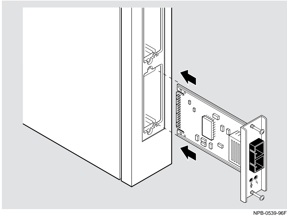
Figure 2-2: Installing the Card
