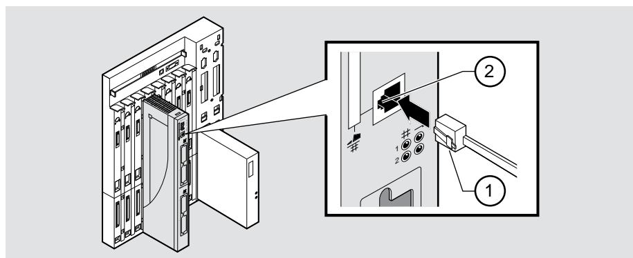
Figure 3-5: LDM Port Cable Connection
