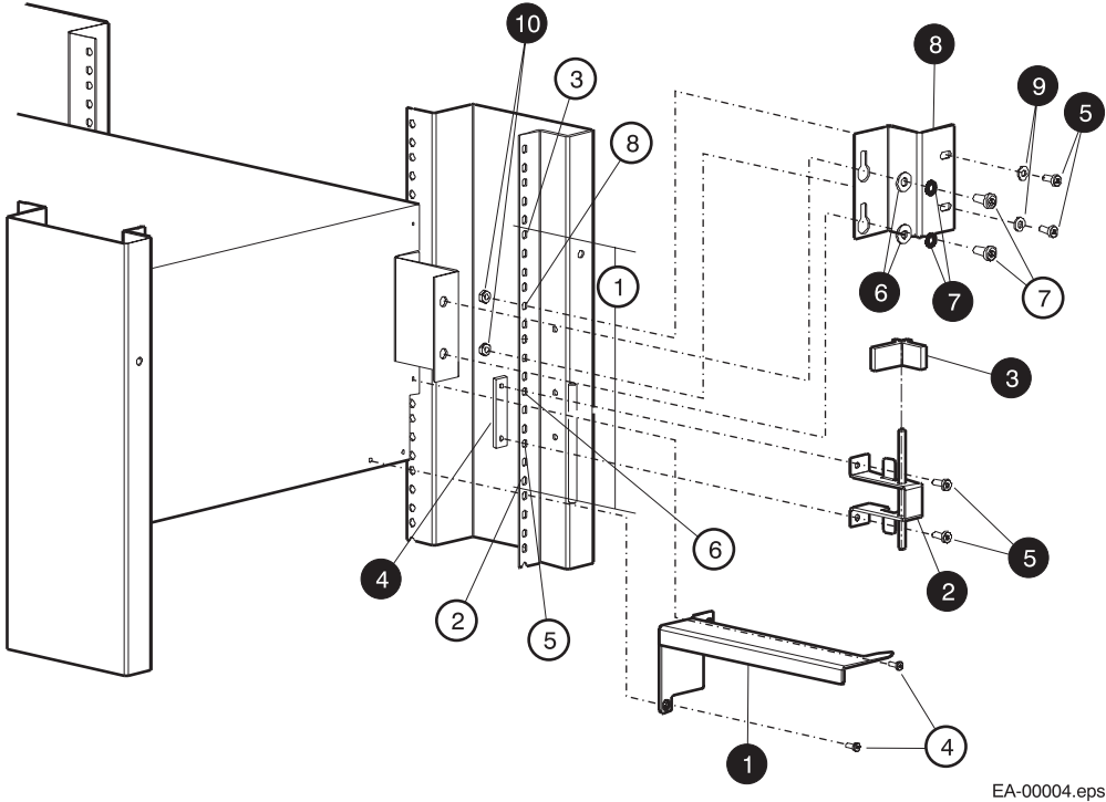
Figure 1 Installing the 2T-PL800-01 Interlock Kit
