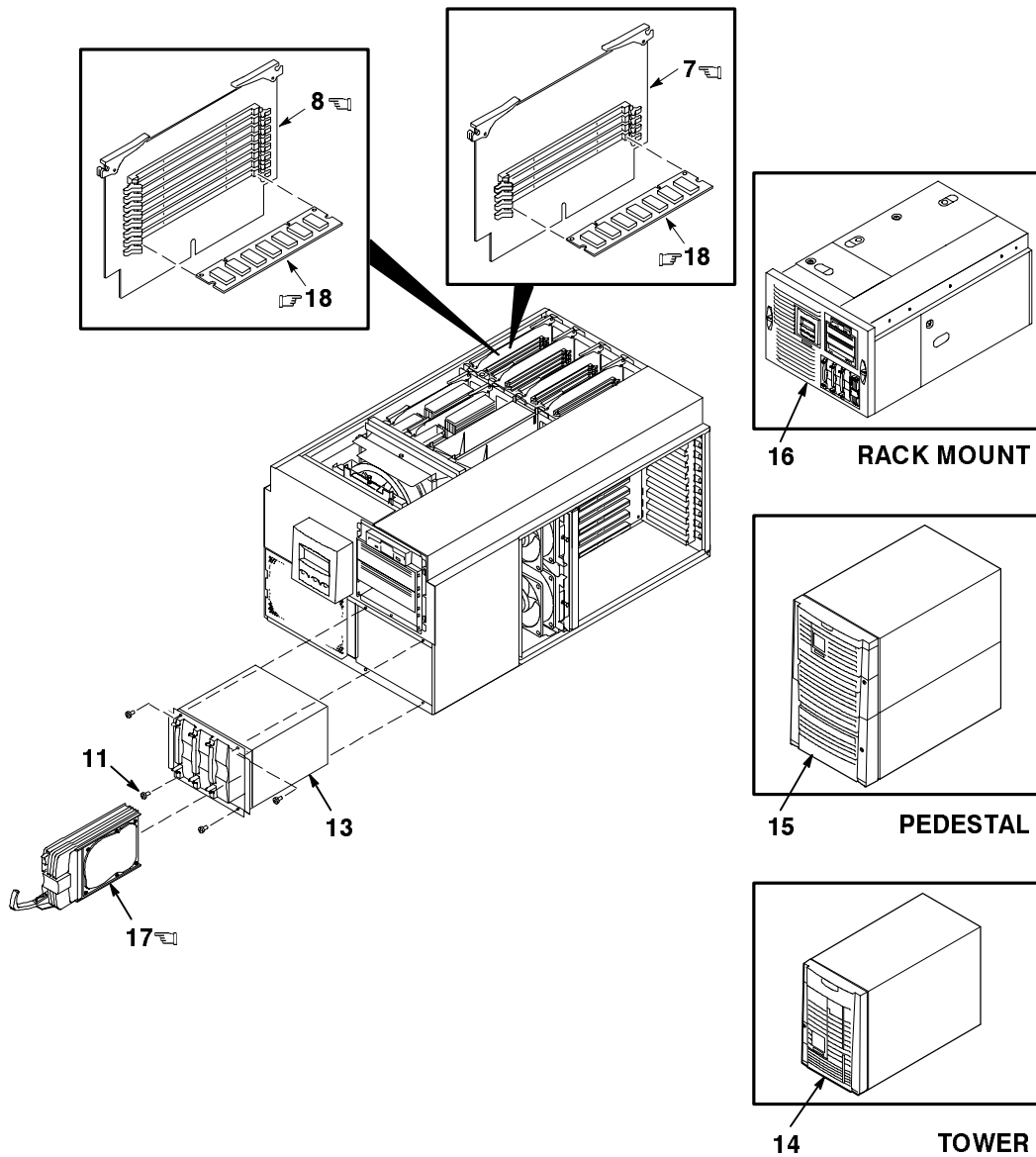
Figure 1. AlphaServer ES40 Kernel Assembly (Sheet 2 of 2)
