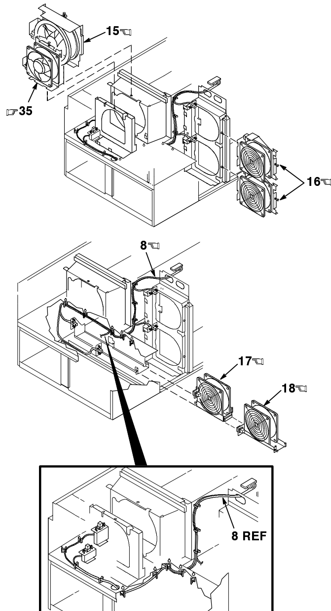
Figure 2. System Box Enclosure Assembly (Sheet 3 of 4)
