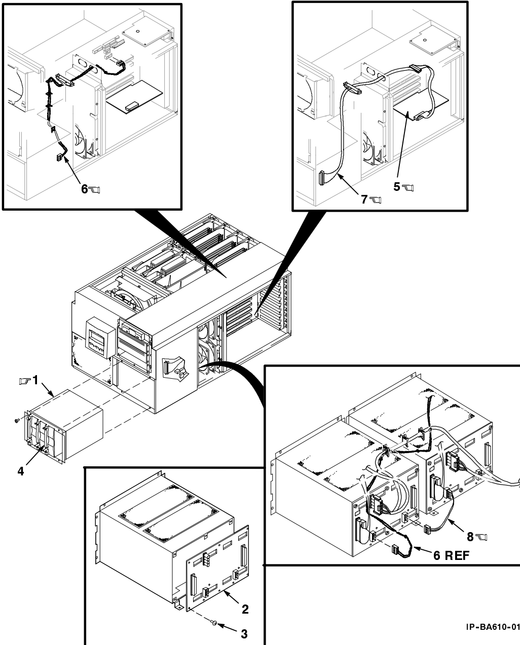
Figure 3. Drive Cage, SCSI, 4 x 1.6 Inch Slots (Sheet 1 of 1)
