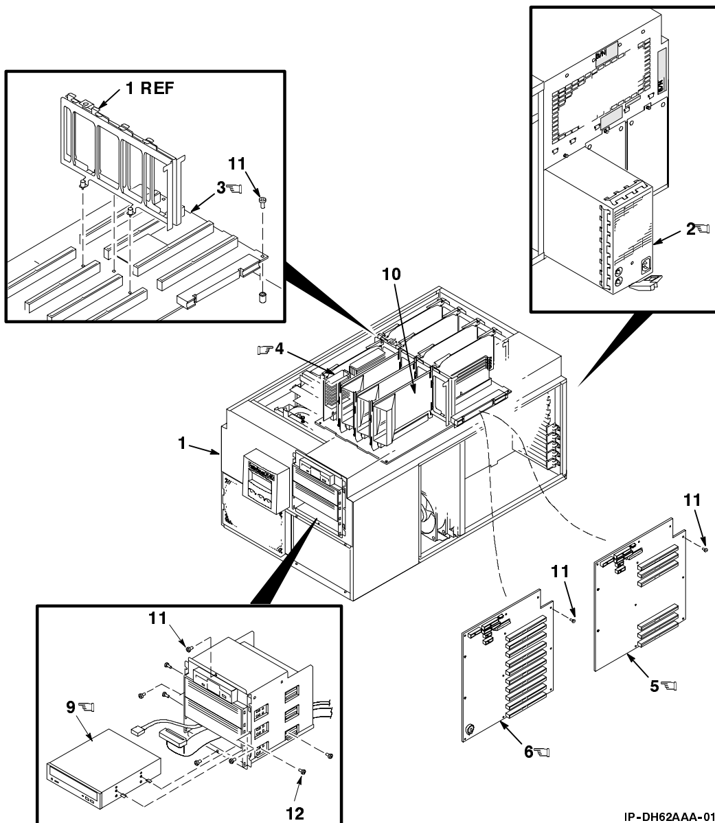
Figure 1. AlphaServer ES40 Kernel Assembly (Sheet 1 of 2)
