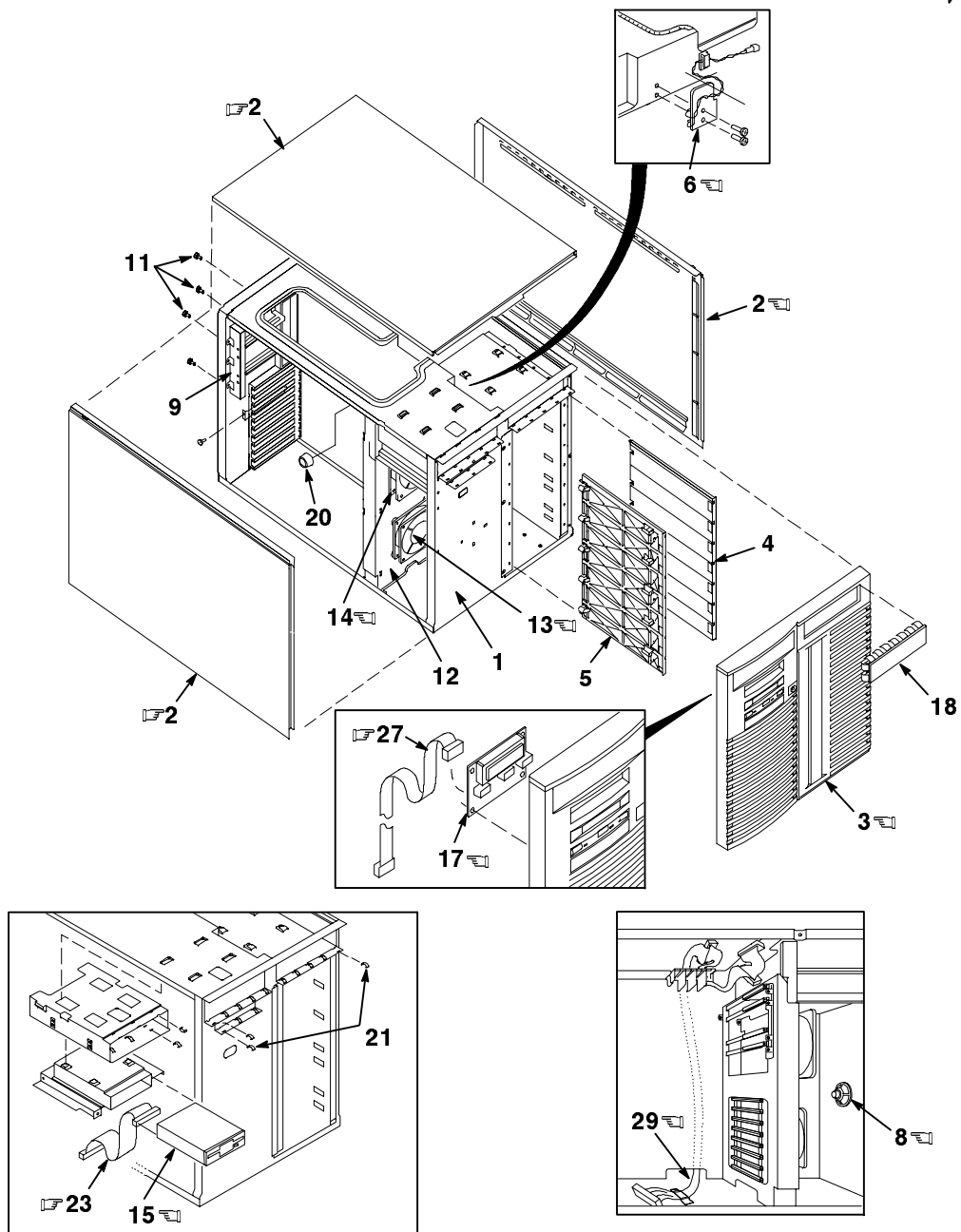
Figure 3. System Box Enclosure Assembly (Sheet 1 of 4)
