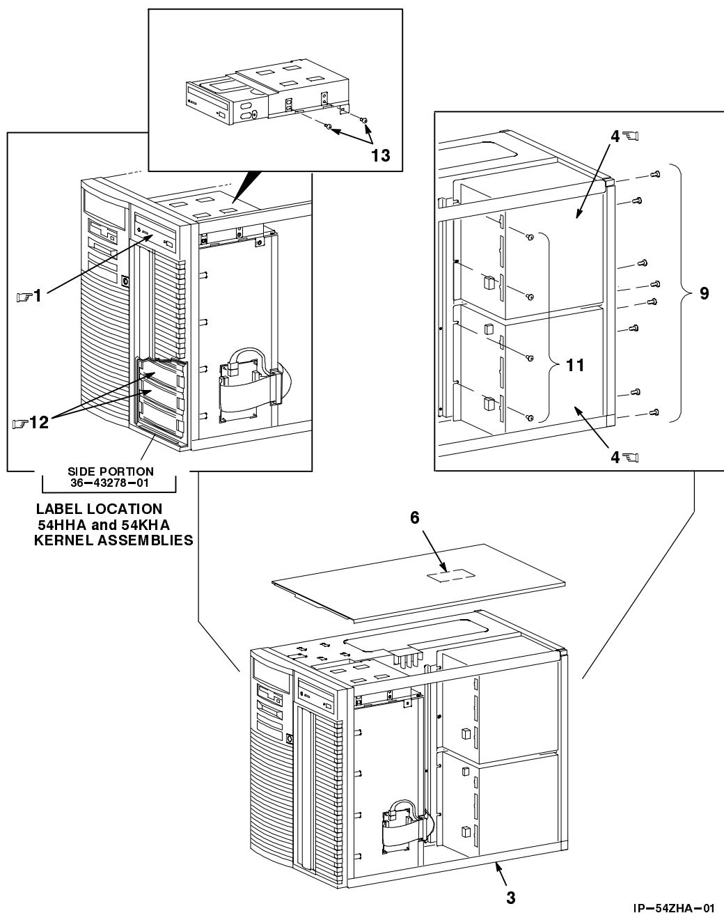
Figure 2. AlphaServer 1200 w/o CPU/Memory or I/O (Sheet 1 of 3)
