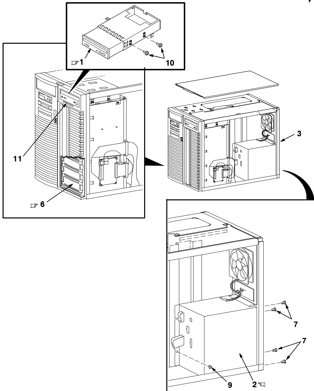
Figure 3. AlphaServer DS20 w/o CPU/Memory or I/O (Sheet 1 of 4) IP-55ZJA-01
