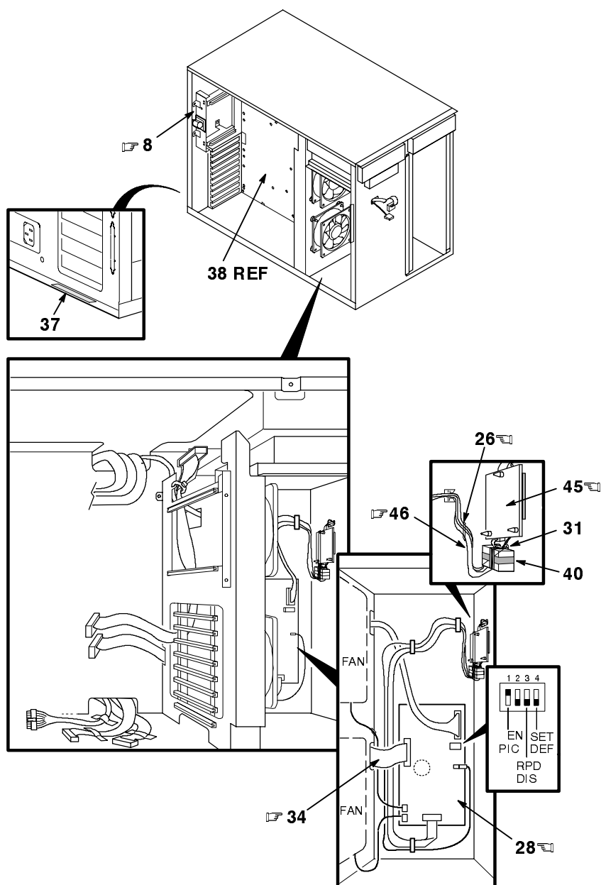
Figure 4. System Box Enclosure Assembly (Sheet 4 of 7)
