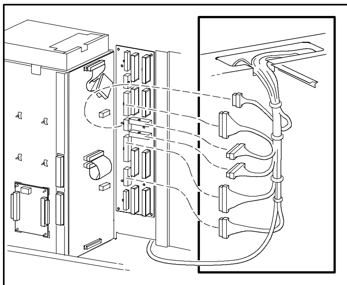
Figure 3. AlphaServer DS20 w/o CPU/Memory or I/O (Sheet 3 of 4)
