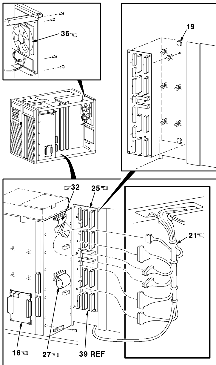
Figure 4. System Box Enclosure Assembly (Sheet 2 of 7)
