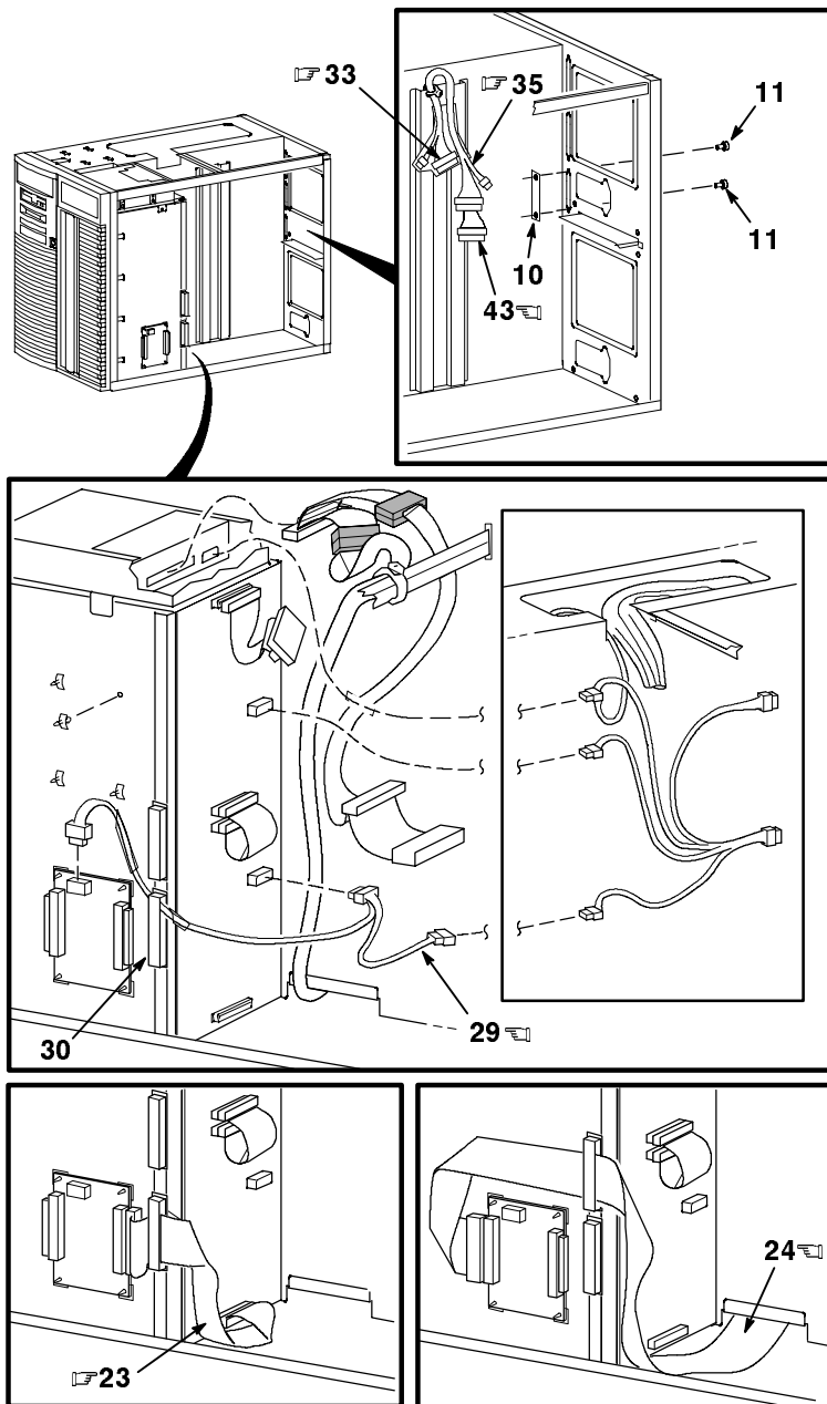
Figure 4. System Box Enclosure Assembly (Sheet 3 of 7)
