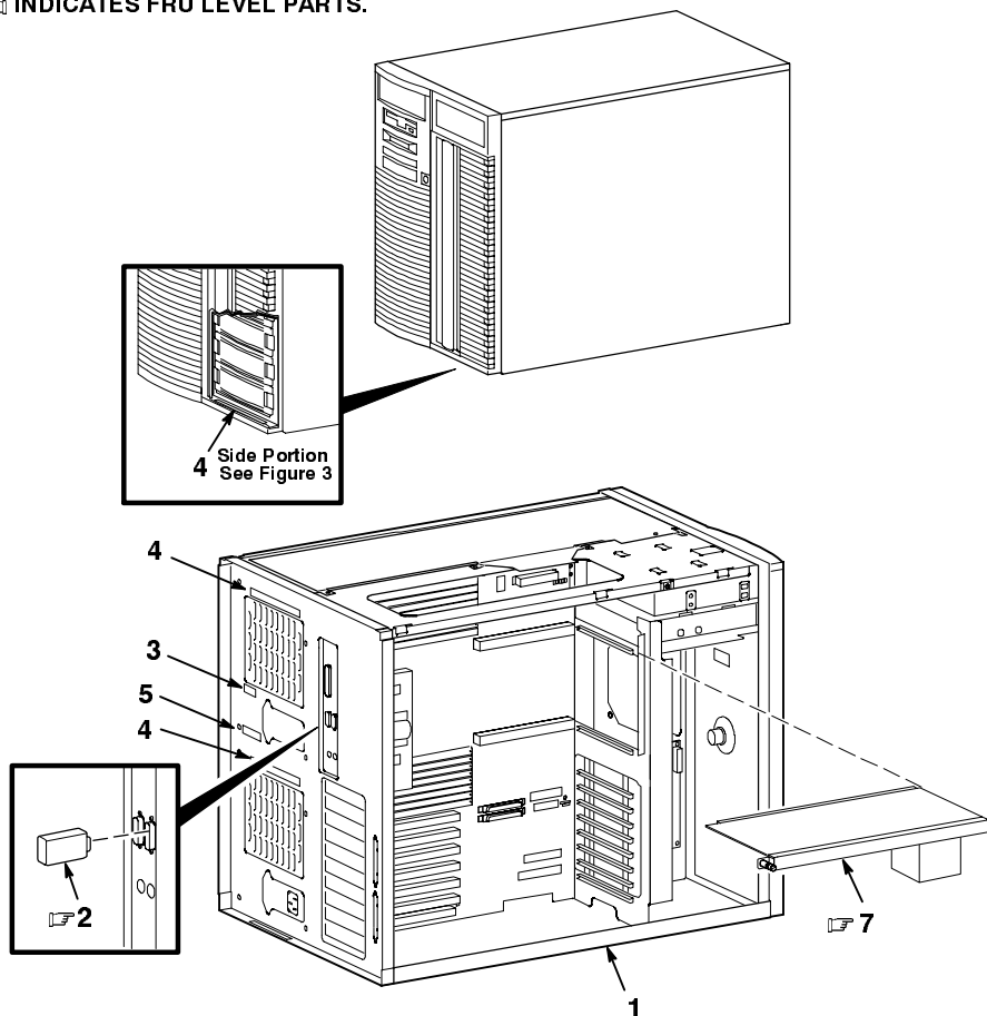
Figure 2. AlphaServer DS20 6/500 Kernel Assembly
