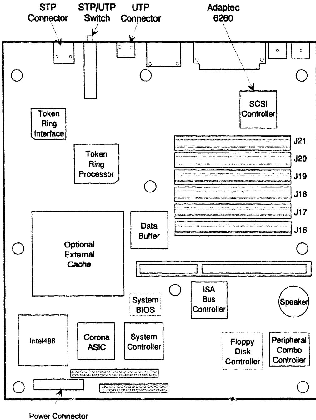
Figure 1-2. DECpc 433 Token Ring Workstation System Board Layout
