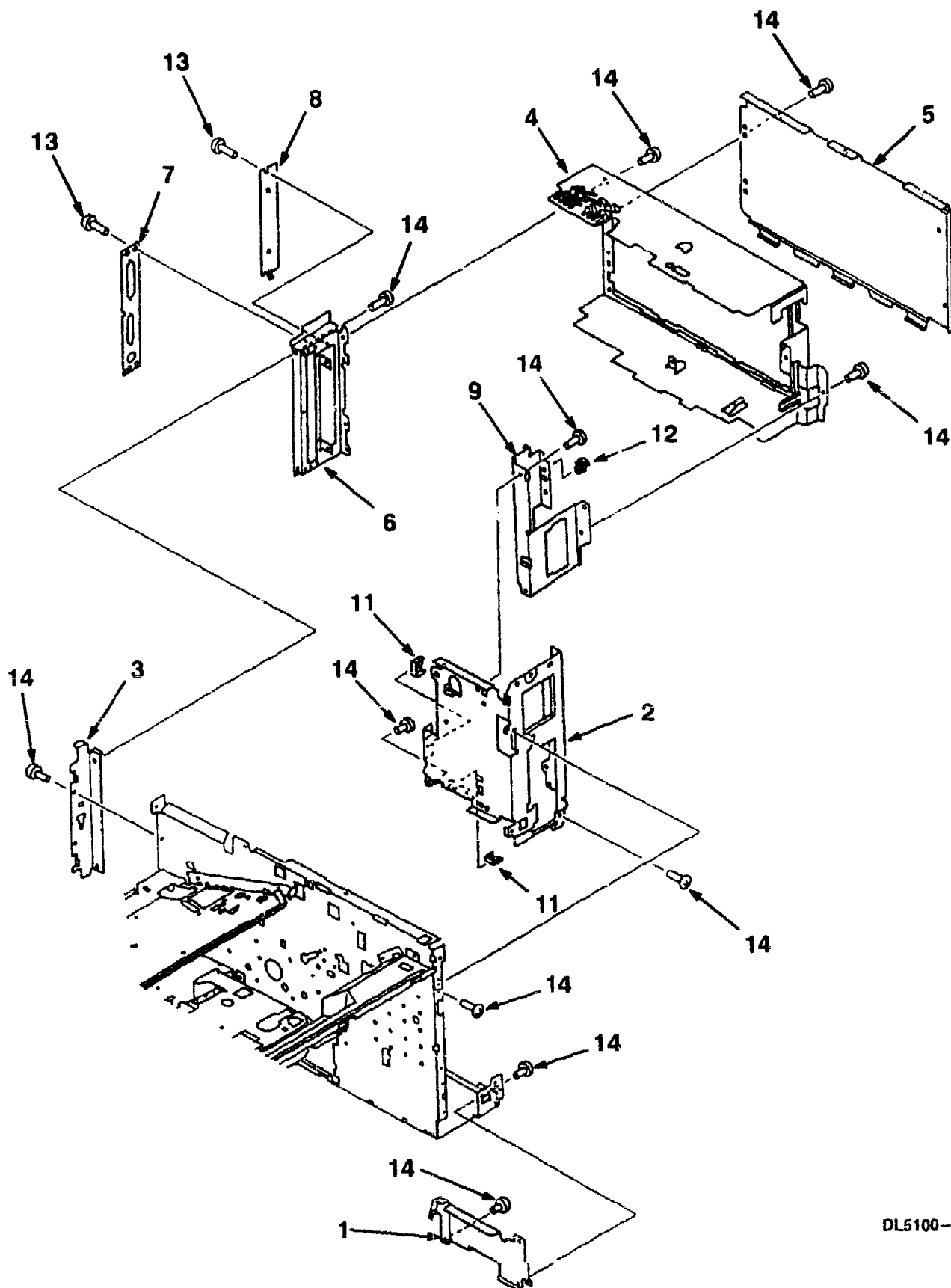
Figure 6. Internal Components (3)
