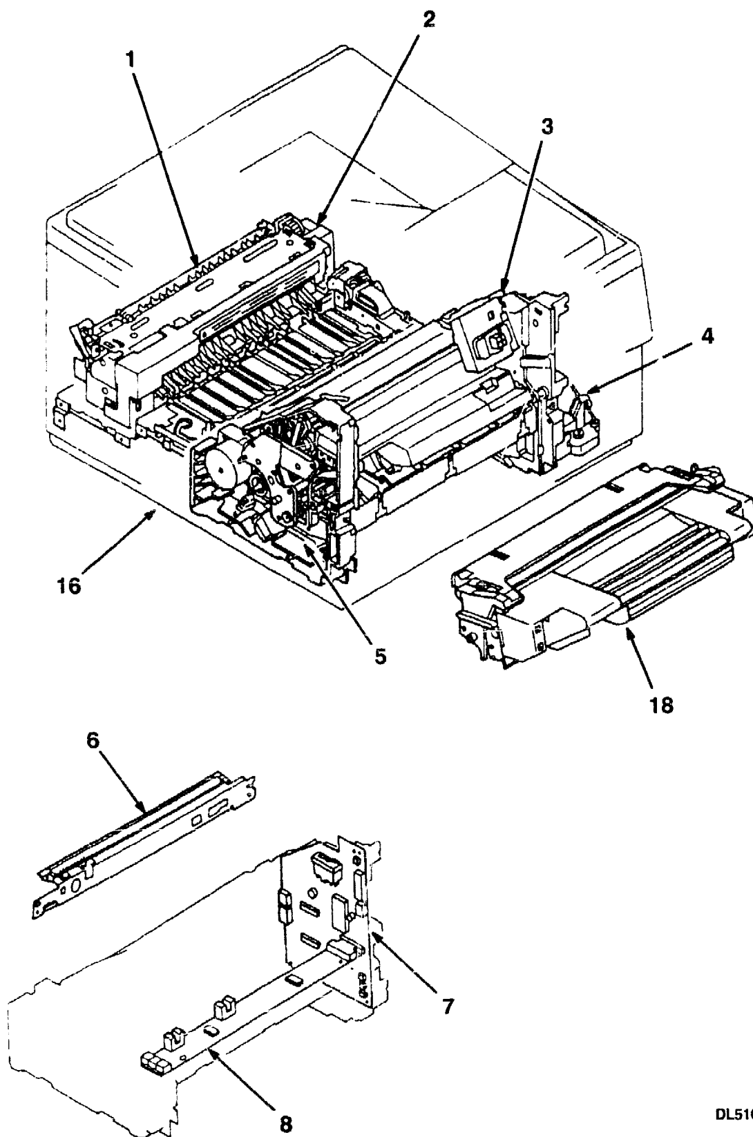
Figure 1. DEClaser 5100 Major Assembly Locations (Sheet 1 to 2)
