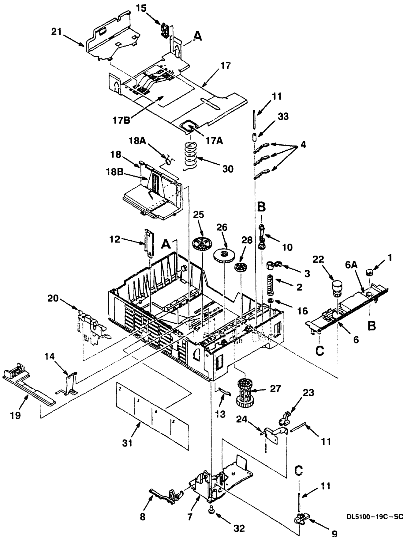
Figure 19C. Tray Assembly, Universal Input - 500 Sheet
