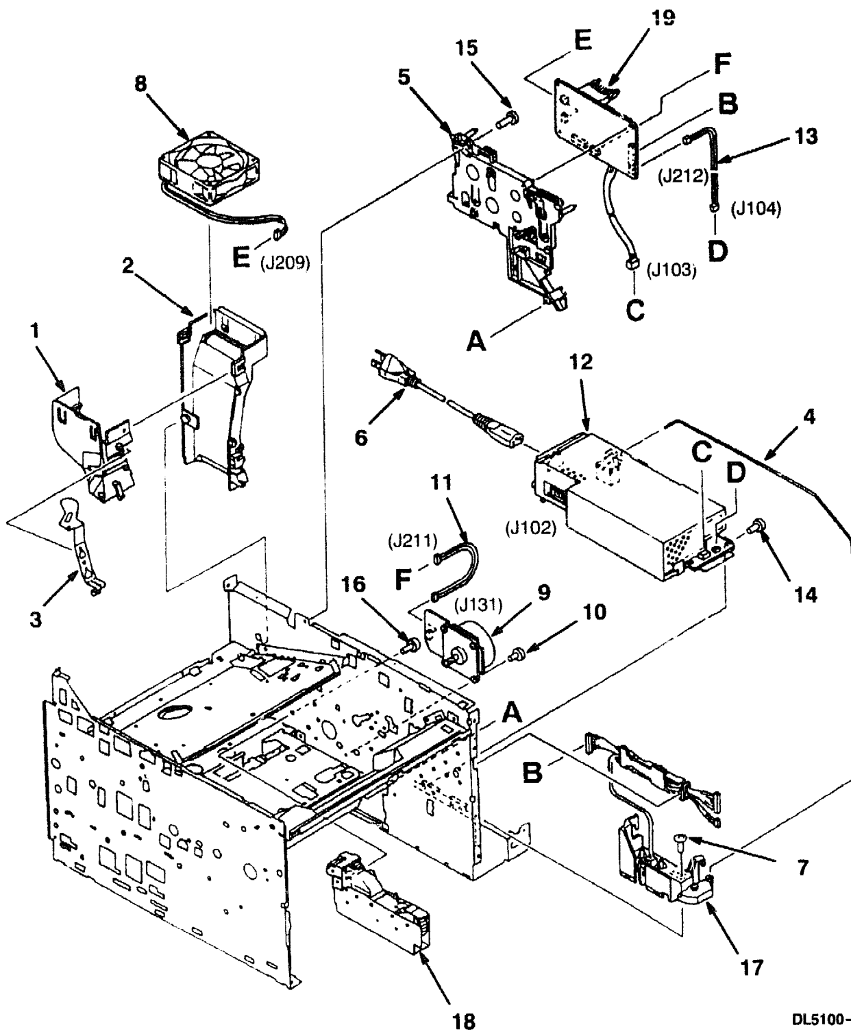
Figure 5. Internal Components (2)
