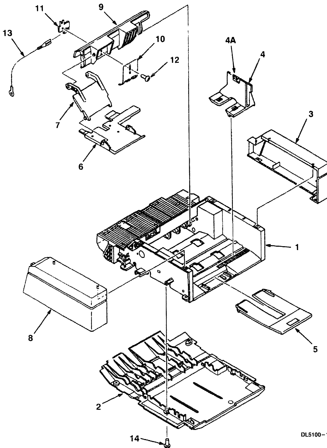
Figure 18A. External Covers, Panels, Etc. – Envelope Feeder
