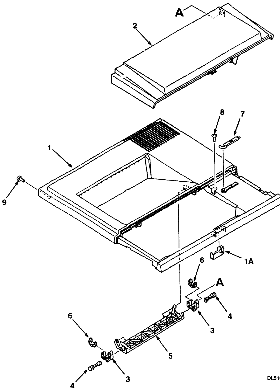
Figure 3. Cover Assembly, Upper
