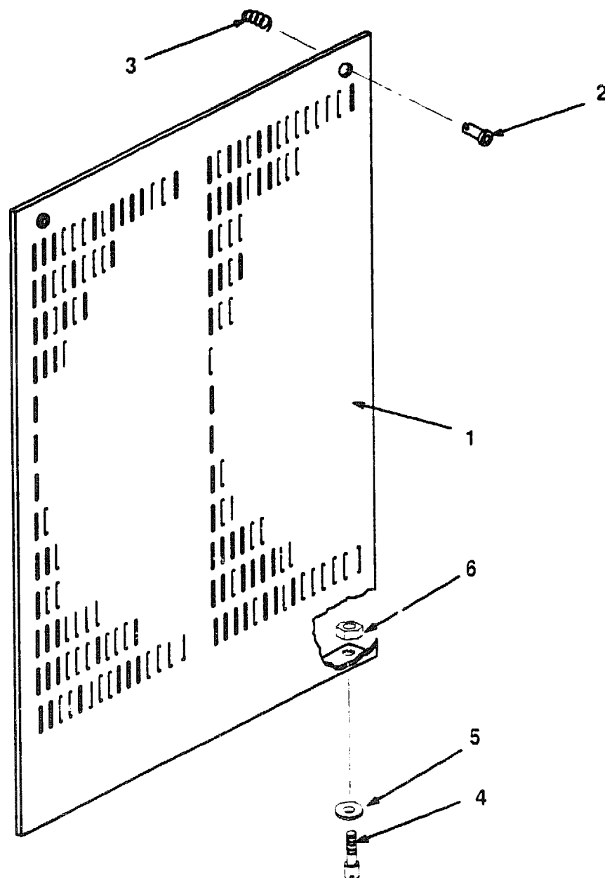
Figure 3. Panel Assembly, SA
