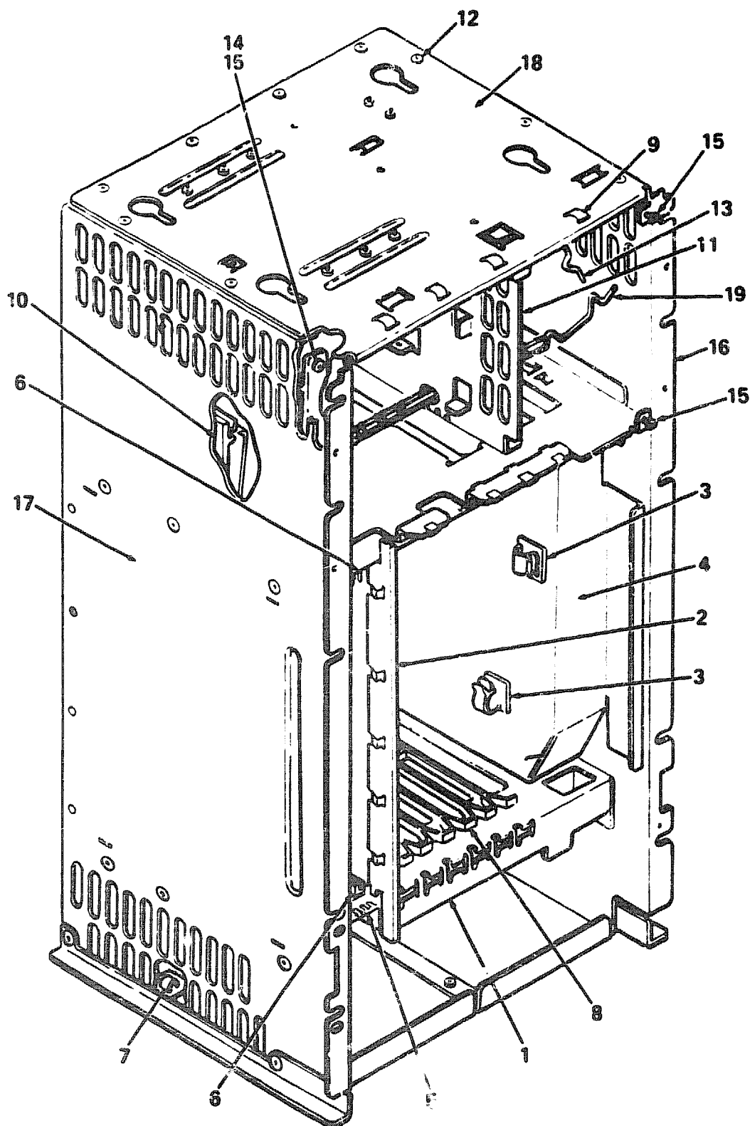
Figure 3. Frame Assembly
