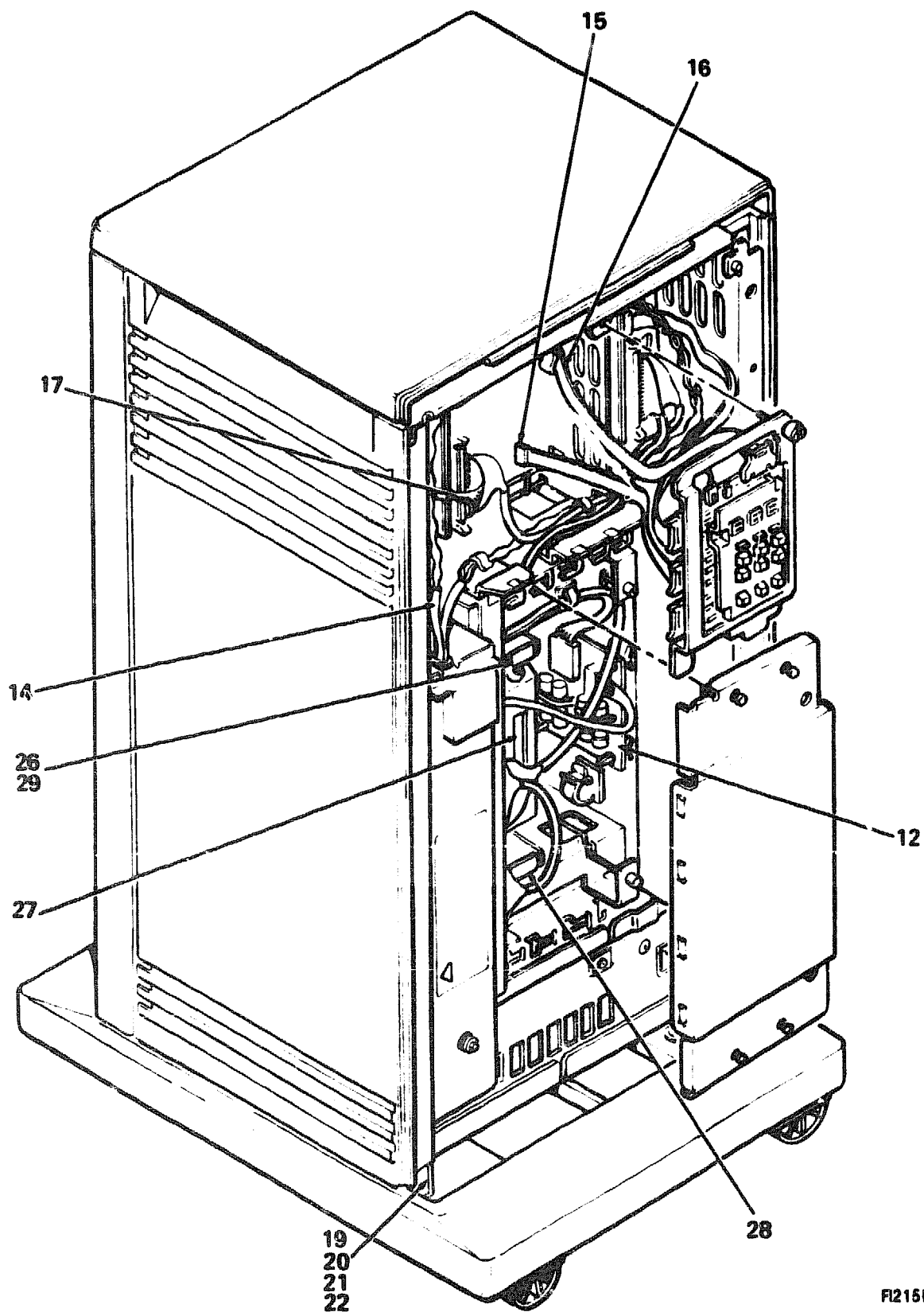
Figure 1. R215F Expander (Sheet 3 of 4)
