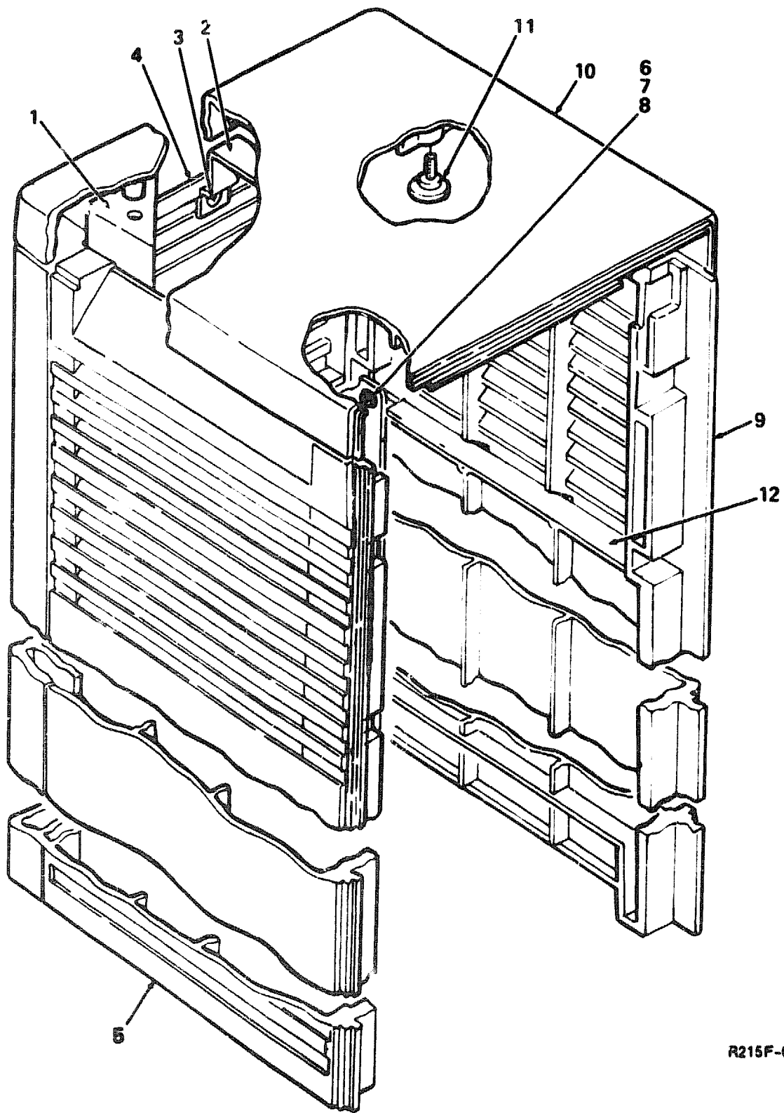
Figure 9. Enclosure Assembly, Shell
