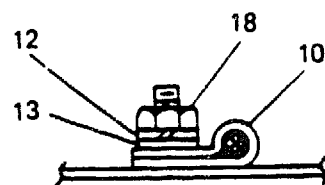
SECTION D-D (ENLARGED) TYPICAL CABLE CLAMP MOUNTING (2 PLACES)
