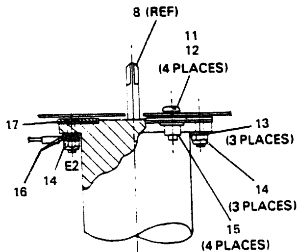
MOTOR MOUNTING DETAIL
