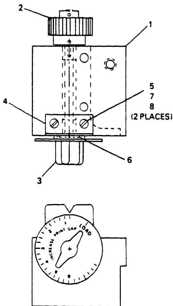
Figure 18. Support Assembly, LH Striker Bar (44C506614-G01) (For Next Higher Assembly, See Figure 14, Item 20)
