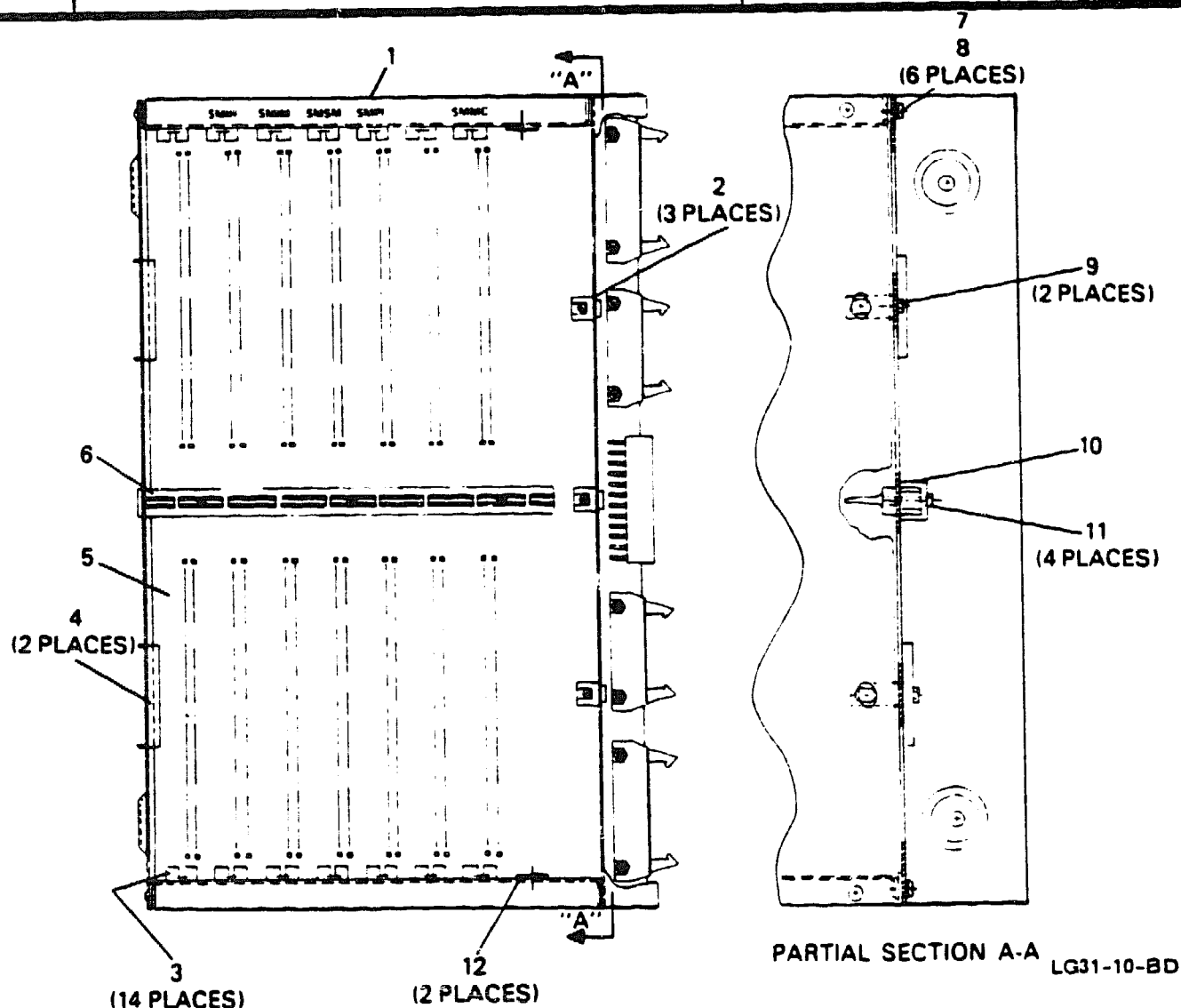
Figure 10. Module Assembly, Logic (44E416564-G01) (For Next Higher Assembly, See Figure 1C, Item 35)
