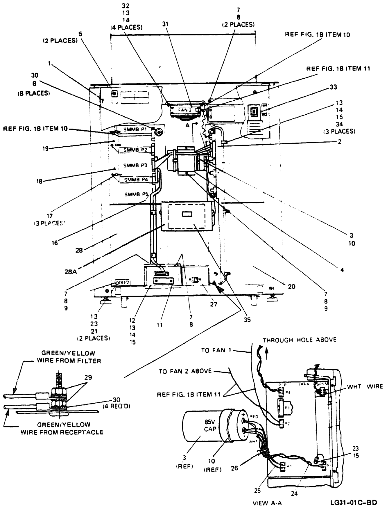
Figure 1D. Printer Assembly (Rear View)
