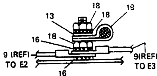
SECTION C-C (ENLARGED)
