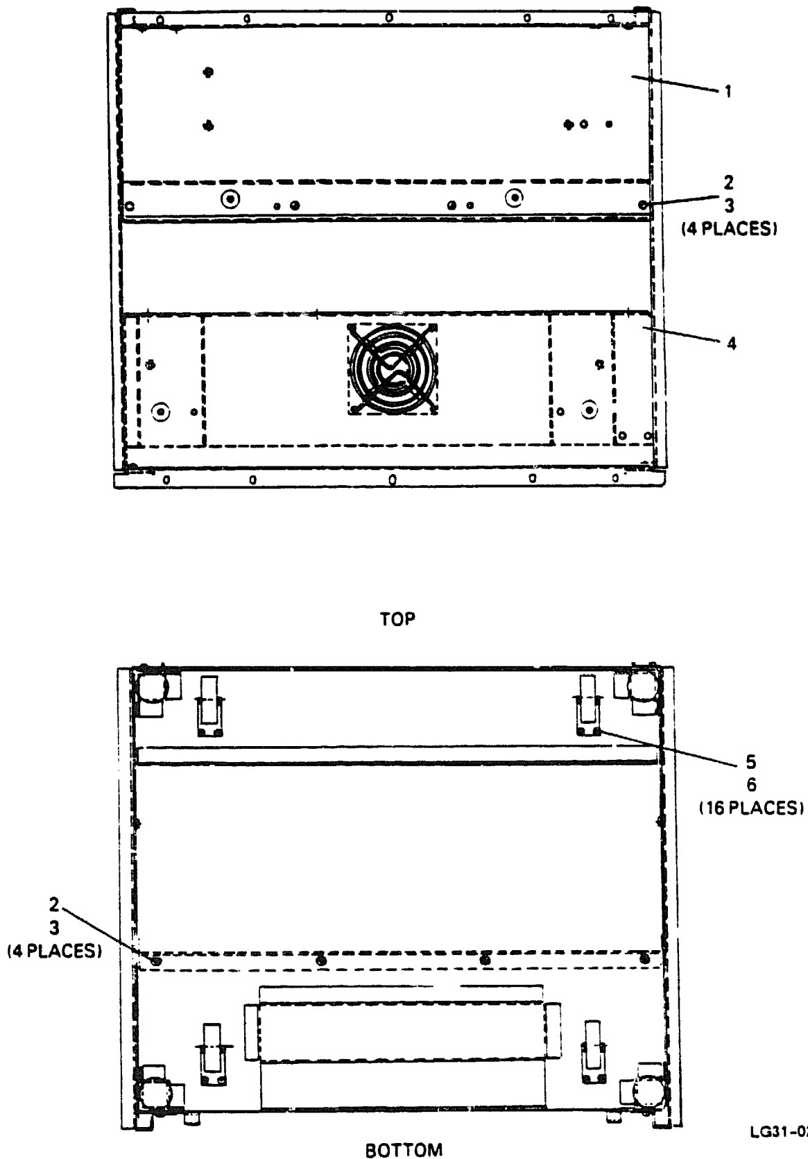
Figure 2B. Enclosure Assembly, Lower (Top And Bottom Views) (44E416566-G101) (See Figure 1A. Item 1)
