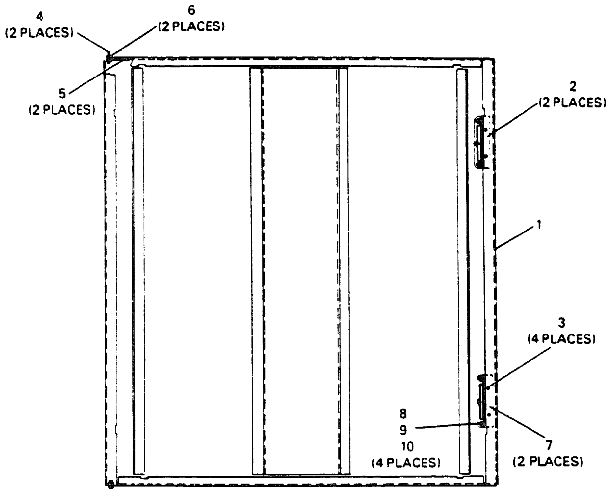
Figure 4. Door Assembly, Front Access (44C505094-G06) (See Figure 1B, Item 12)
