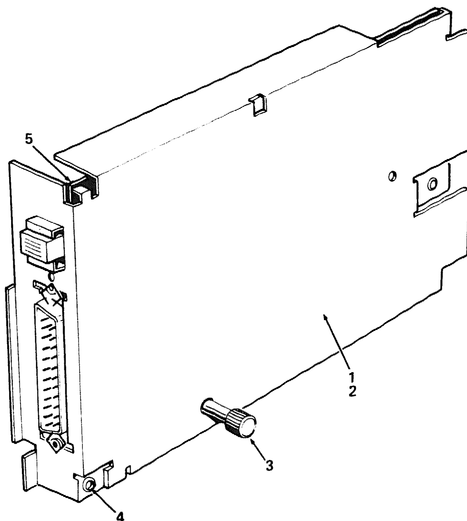
Figure 6. Interface Module Assembly, LA324 PAR/SER
