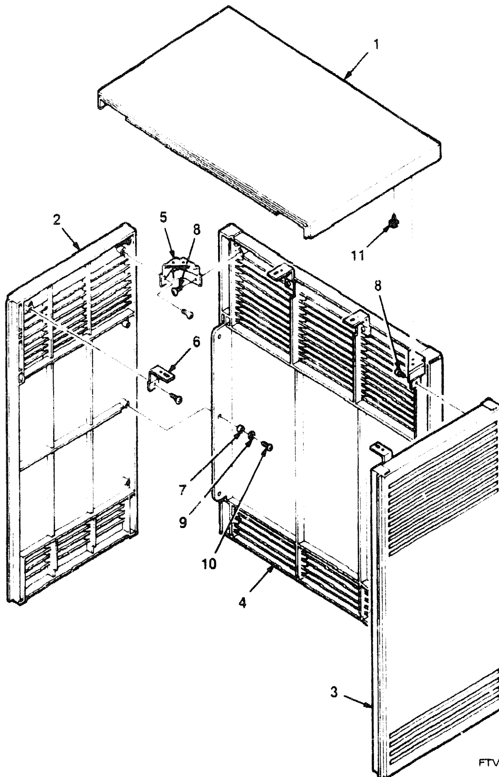
Figure 14. Enclosure Assembly, Shell
