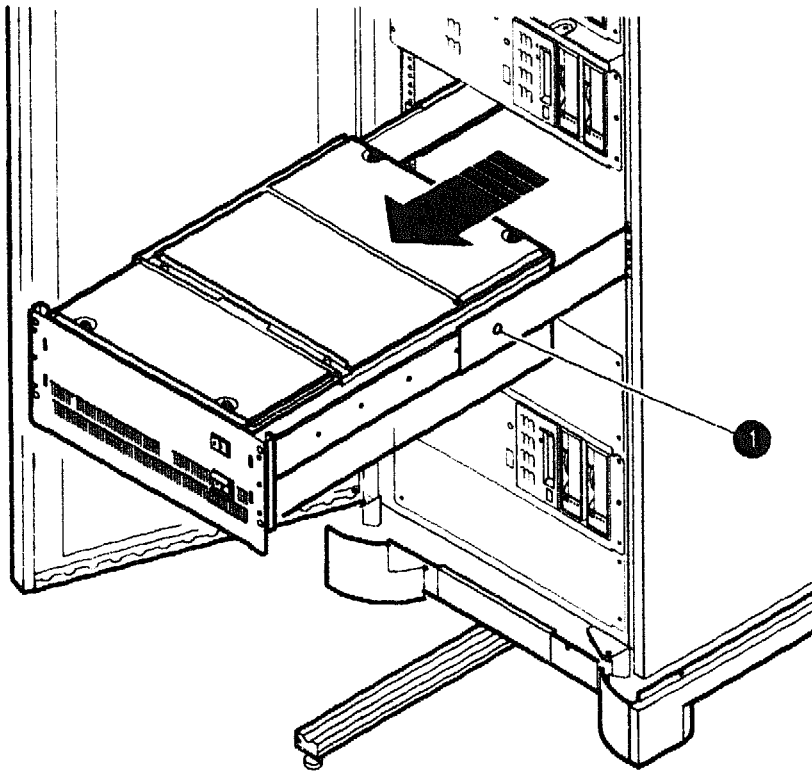
Figure 3-31 Removing the CPU Drawer
