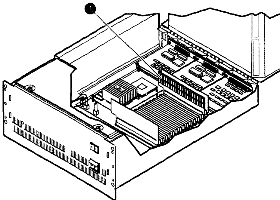
Figure 3–20 Removing the MS02-CA Memory Module
