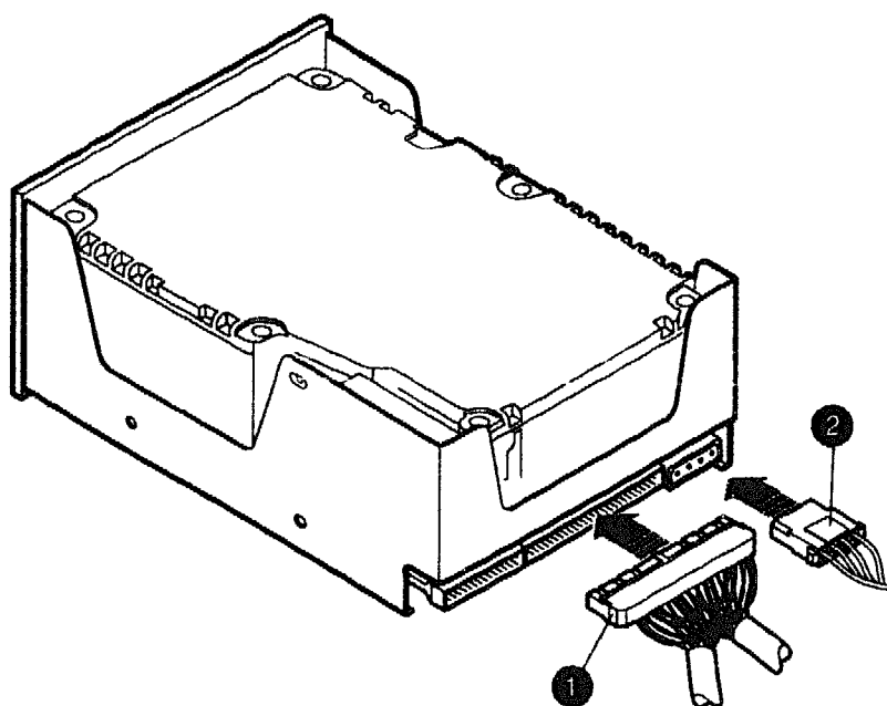
Figure 4–35 Disconnecting/Connecting an RZ58
