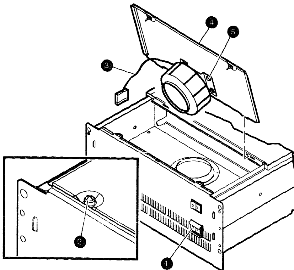
Figure 3-12 Removing the CPU Drawer Blower
