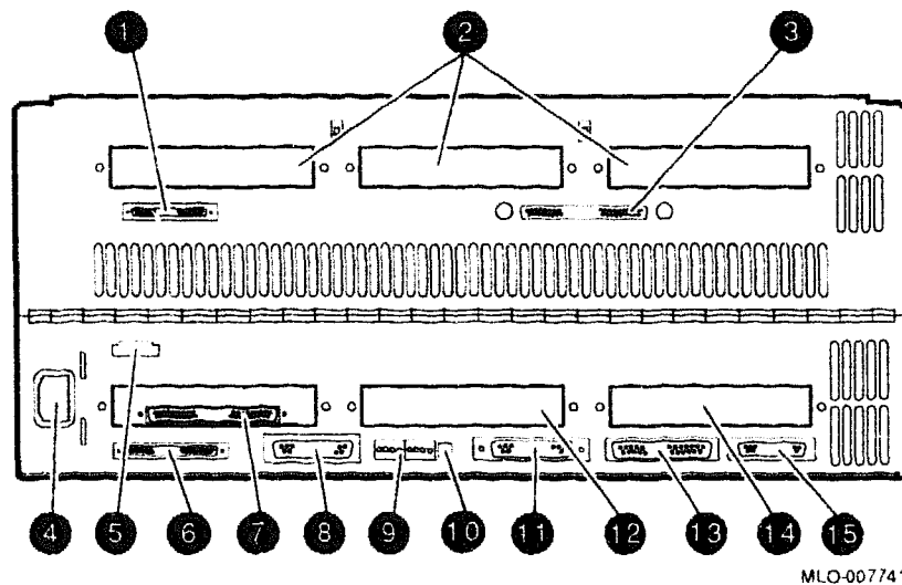
Figure 1-7 CPU Drawer Rear Panel
