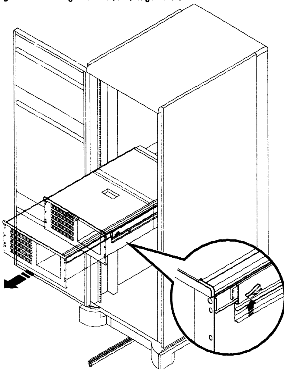
Figure 4-3 Pulling Out a Mass Storage Drawer
