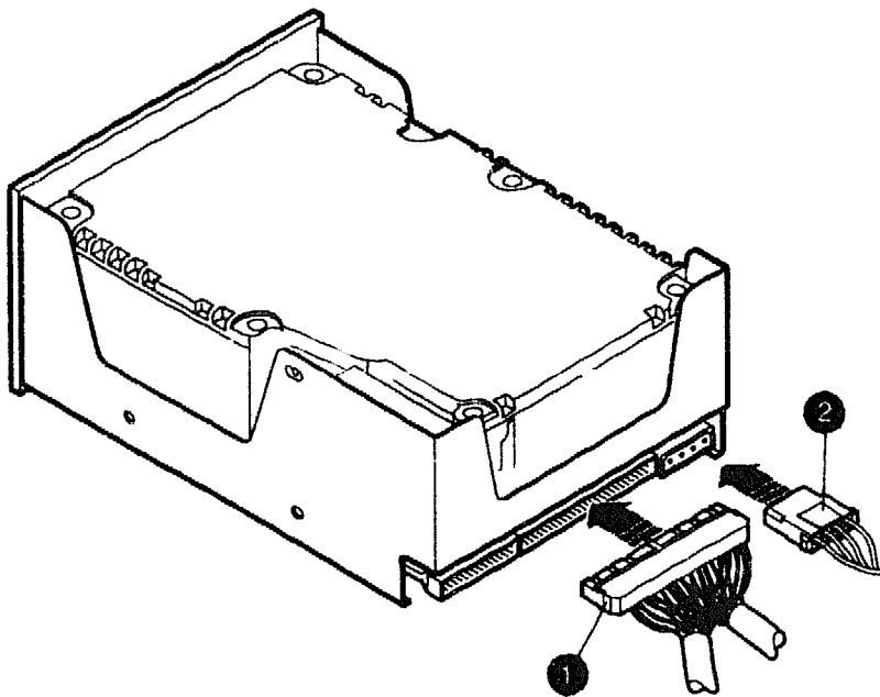
Figure 4-32 Disconnecting/Connecting an R257
