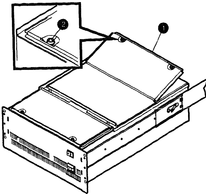
Figure 3-11 Opening the CPU Drawer Rear Top Cover
