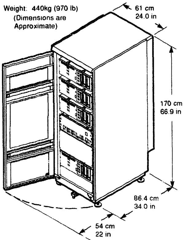
Figure 2-1 DECsystem 5900 Enclosure Dimensions
