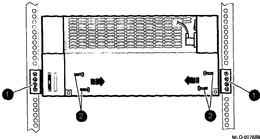
Figure 2-10 Mass Storage Drawer Bracket Screws
