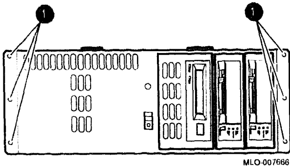
Figure 4-2 Removing Drawer Front Hex Screws
