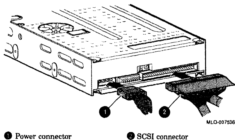
Figure 4-54 Disconnecting/Connecting a TZK10
