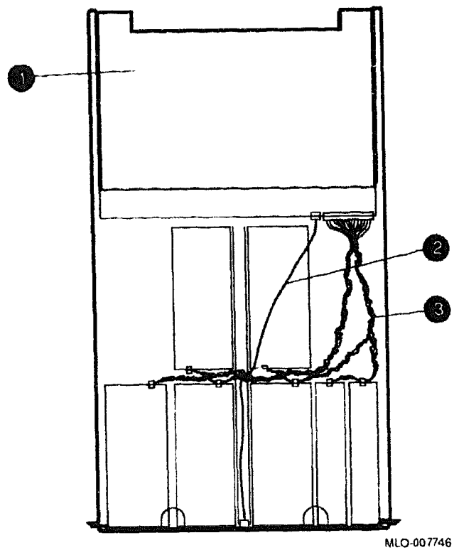
Figure 1-16 Mass Storage Drawer 1 Power Supply and Harness
