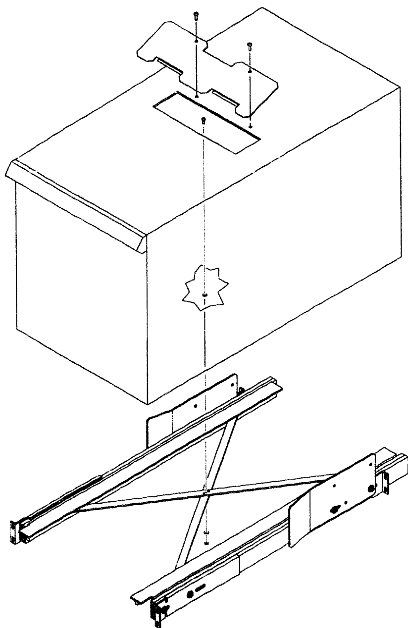
Figure 4-68 Removing the StorageServer 100 from the Cabinet
