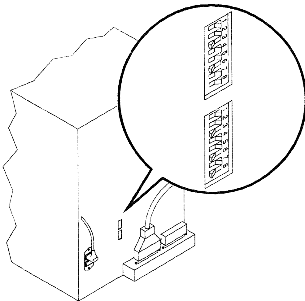
Figure 4-57 External StorageServer 100 SCSI ID Switches
