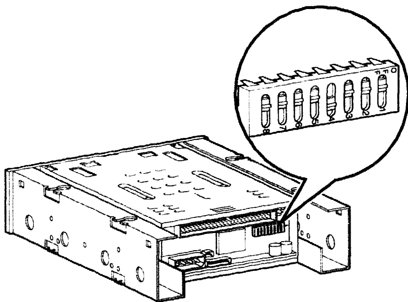
Figure 4-49 SCSI ID Switches on a TLZ06
