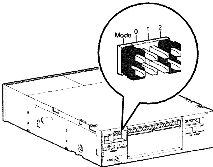
Figure 4-38 SCSI ID Jumpers on an RRD42
