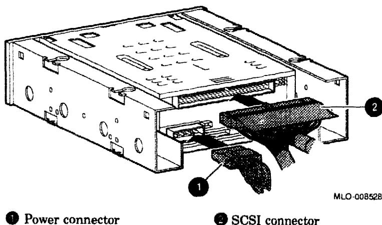
Figure 4-48 Disconnecting/Connecting a TLZ06
