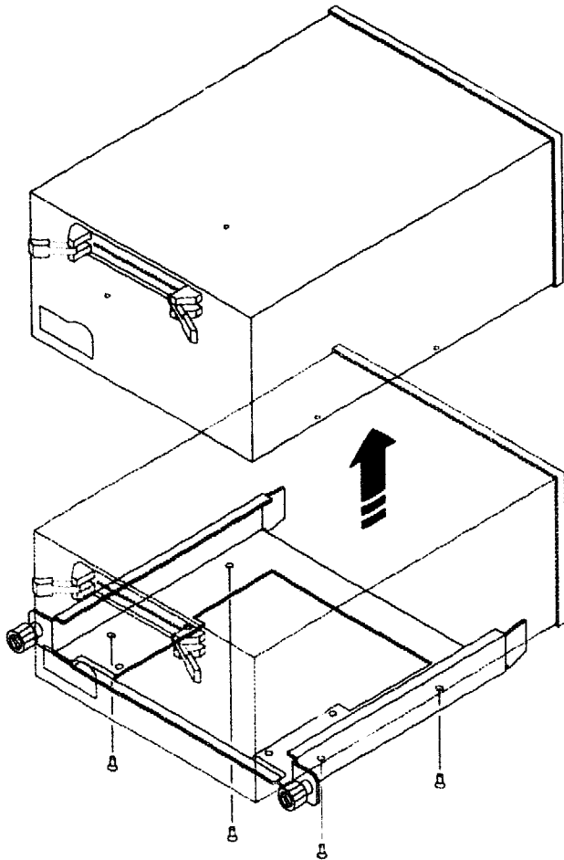
Figure 4-20 Removing a Device from a Bracket
