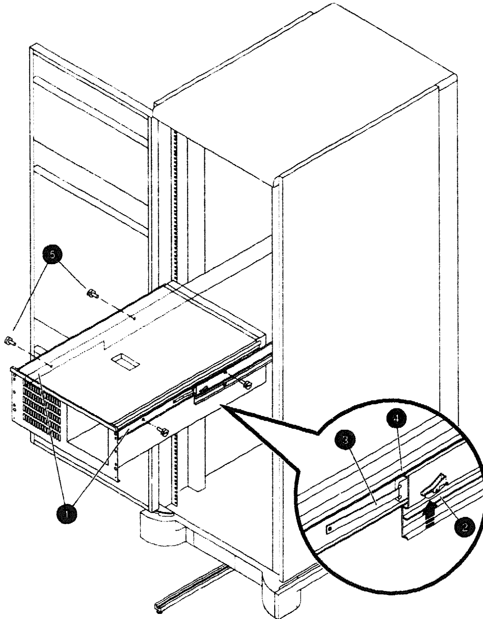
Figure 4-73 Removing a Mass Storage Drawer 2
