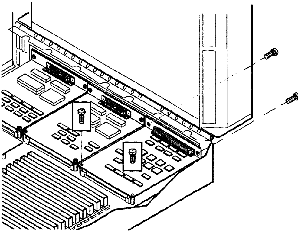
Figure 3-22 Removing a TURBOchannel Option
