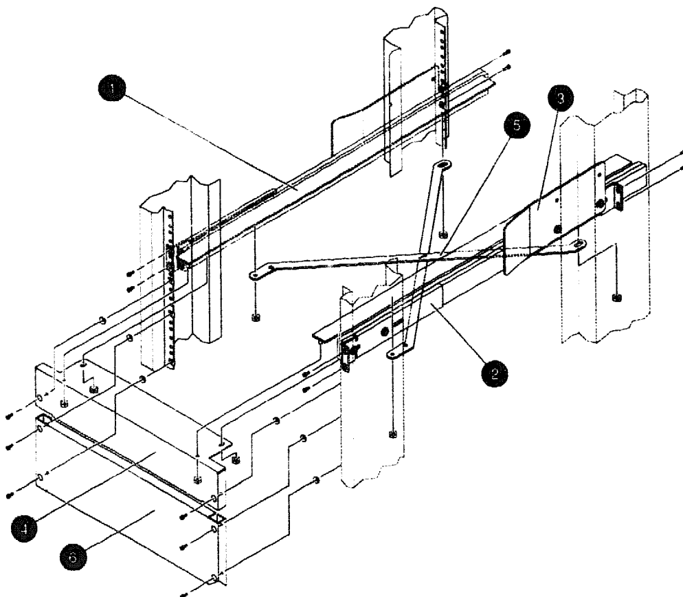
Figure 4-71 Assembling and Installing the Rackmounted Slide Assembly
