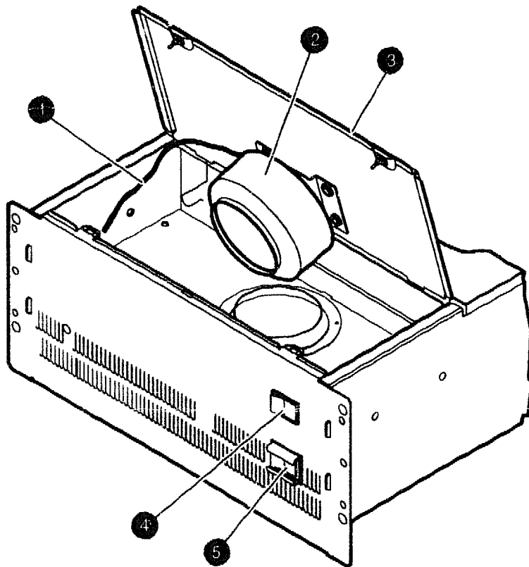
Figure 1-9 CPU Drawer Blower
