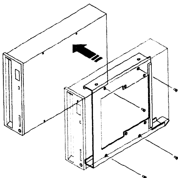
Figure 4-25 Removing a Half-Height Device from a Mass Storage Drawer 2 Removable Media Device Bracket
