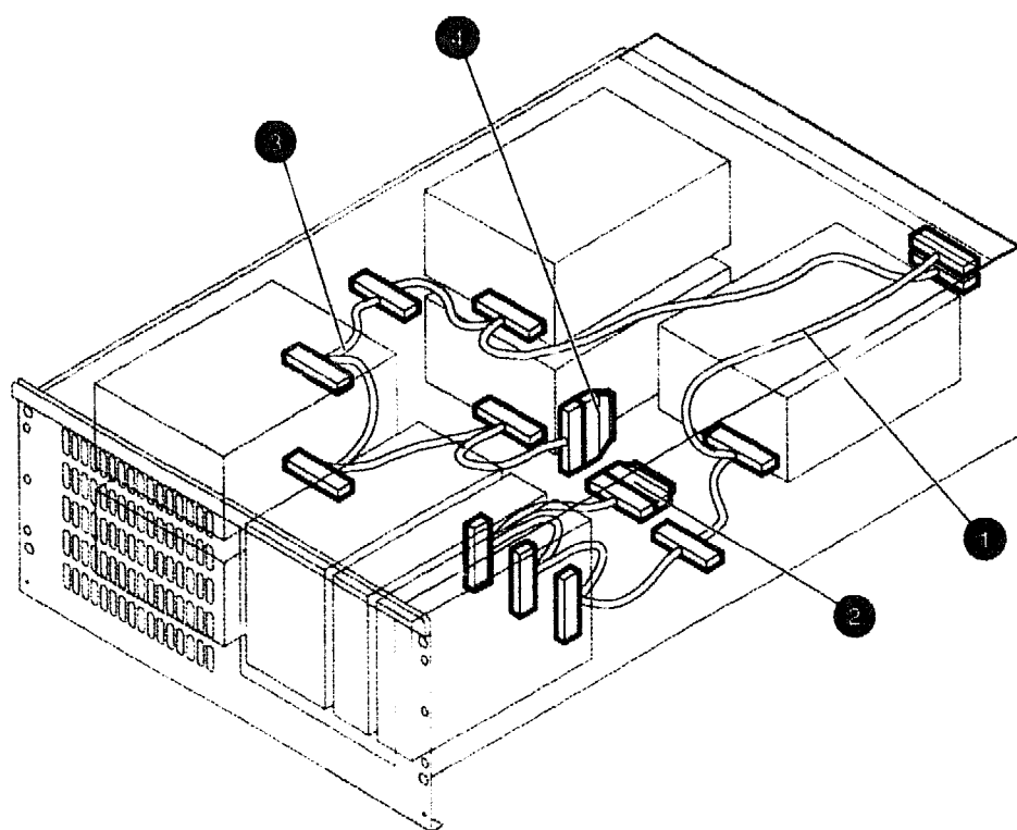
Figure 4–31 Split Bus Configuration for Mass Storage Drawer 2
