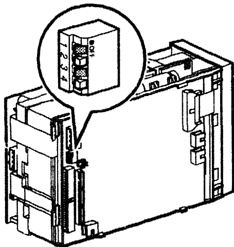
Figure 4-53 SCSI ID Switches on an Internal TZ85
