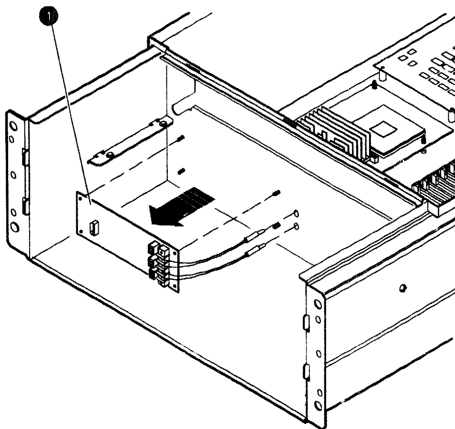
Figure 3-17 Removing the Power Distribution Module
