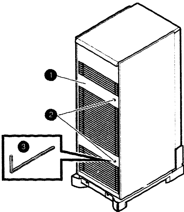
Figure 2-7 Opening the Front Enclosure Door
