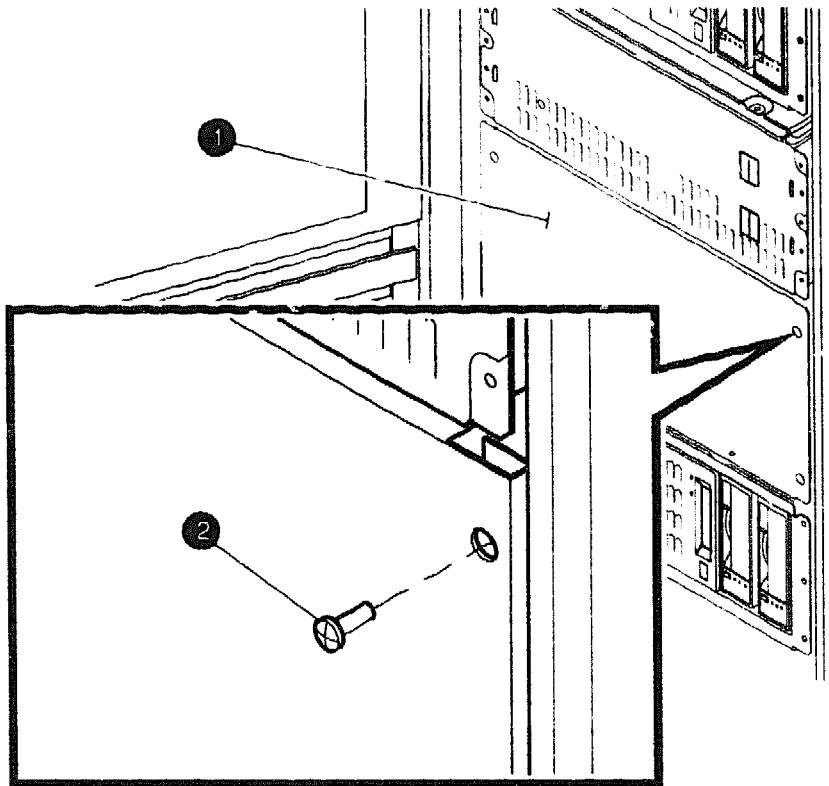
Figure 4-1 Removing Filler Panel(s)
