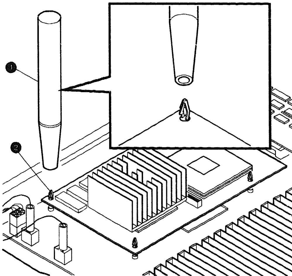
Figure 3-18 Removing the CPU/Daughter Card
