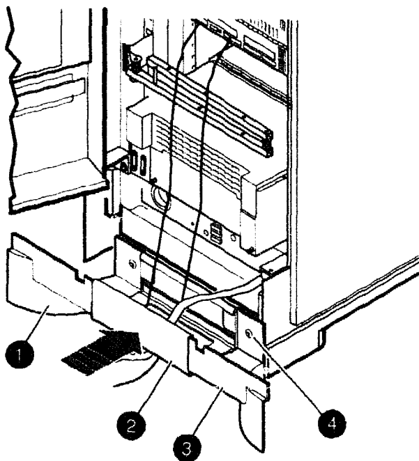
Figure 2-5 Rear Skirt
