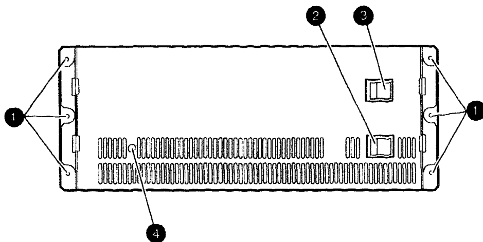
Figure 1-6 CPU Drawer Front Panel
