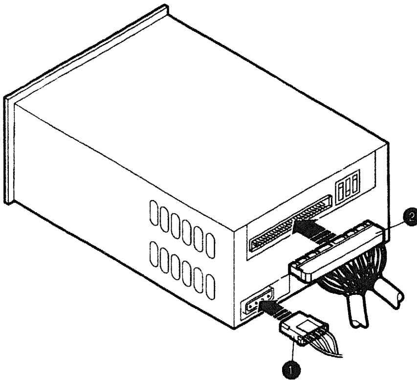
Figure 4-44 Disconnecting/Connecting an Internal TKZ09
