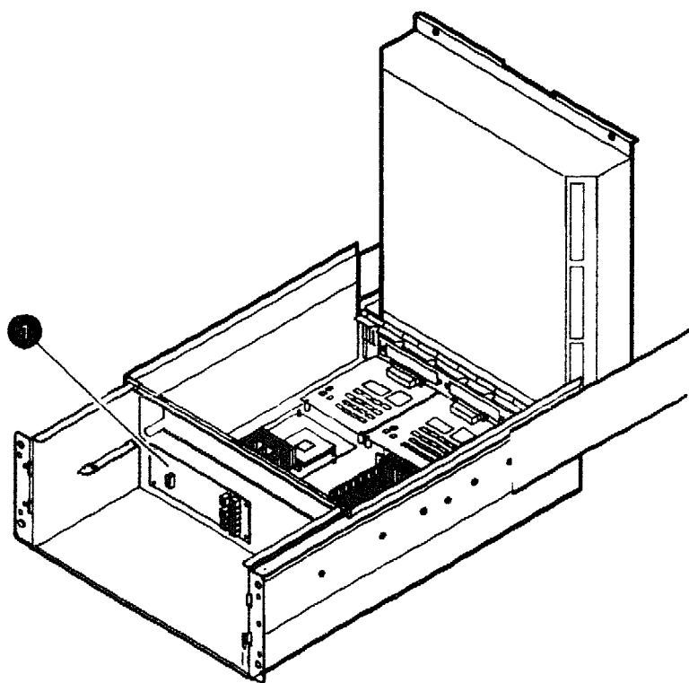
Figure 3-14 Locating the Power Distribution Module
