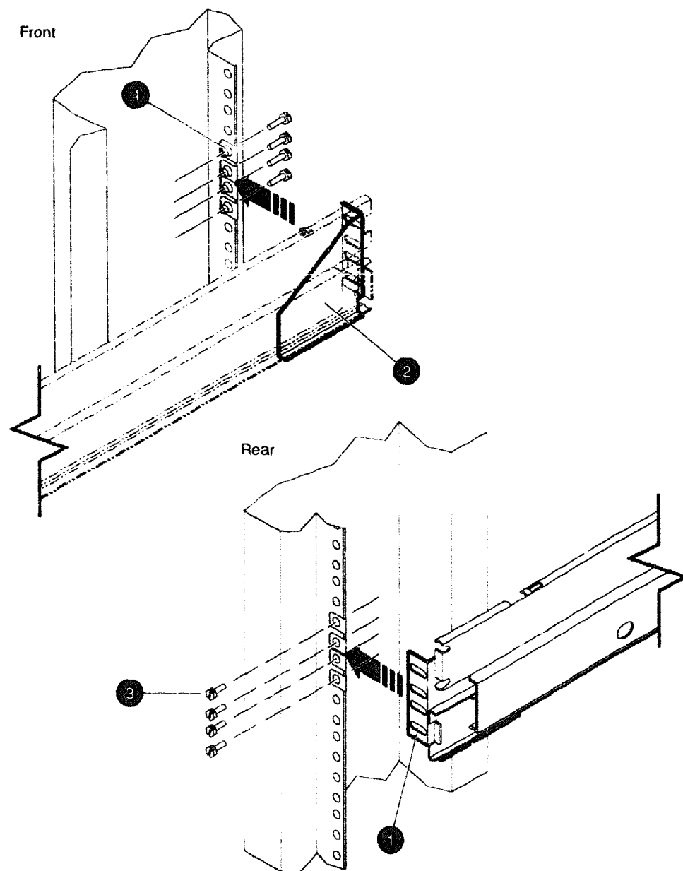
Figure 4-75 Installing Mass Storage Drawer Slides
