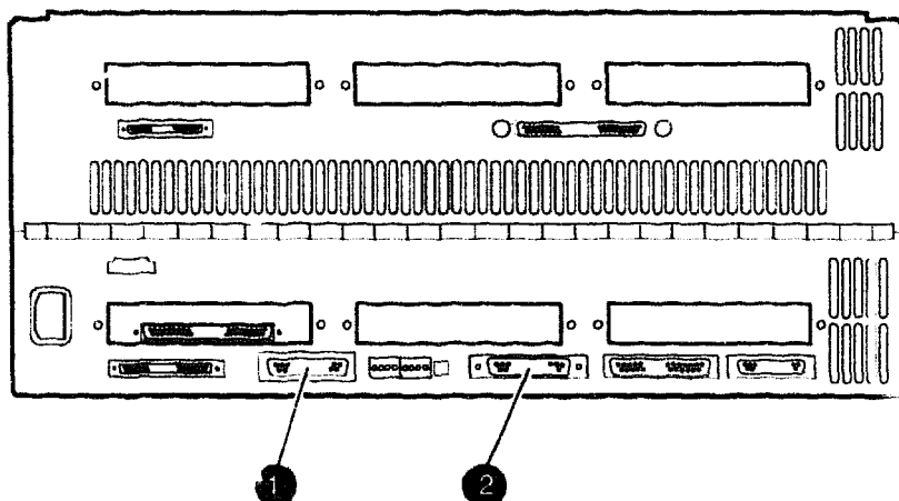
Figure 2-12 Connecting the Console Terminal and Ethernet Cables
