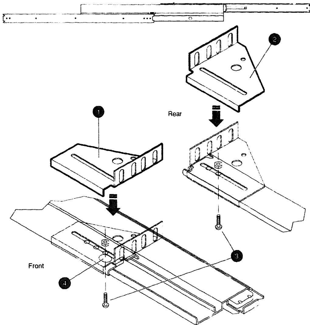
Figure 4-74 Assembling Mass Storage Drawer Slides
