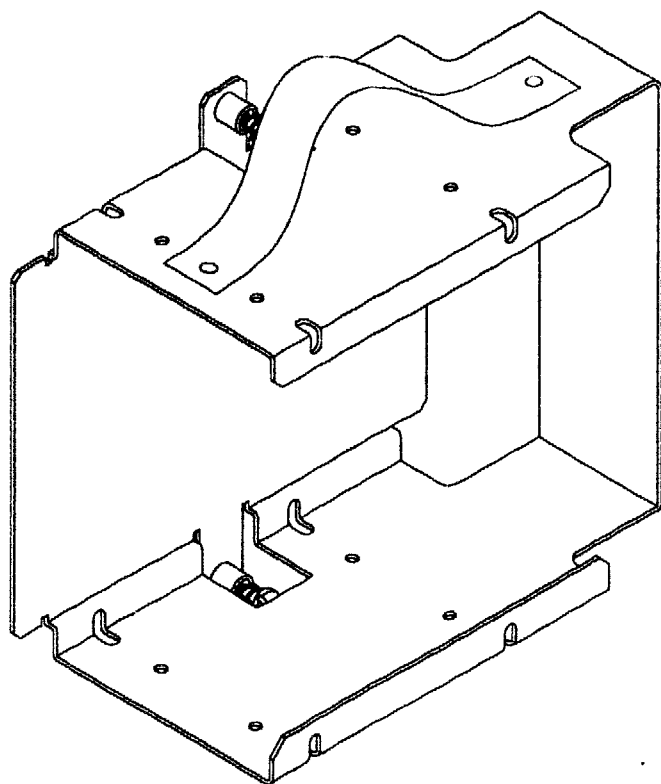
Figure 4-6 Drive Bracket
