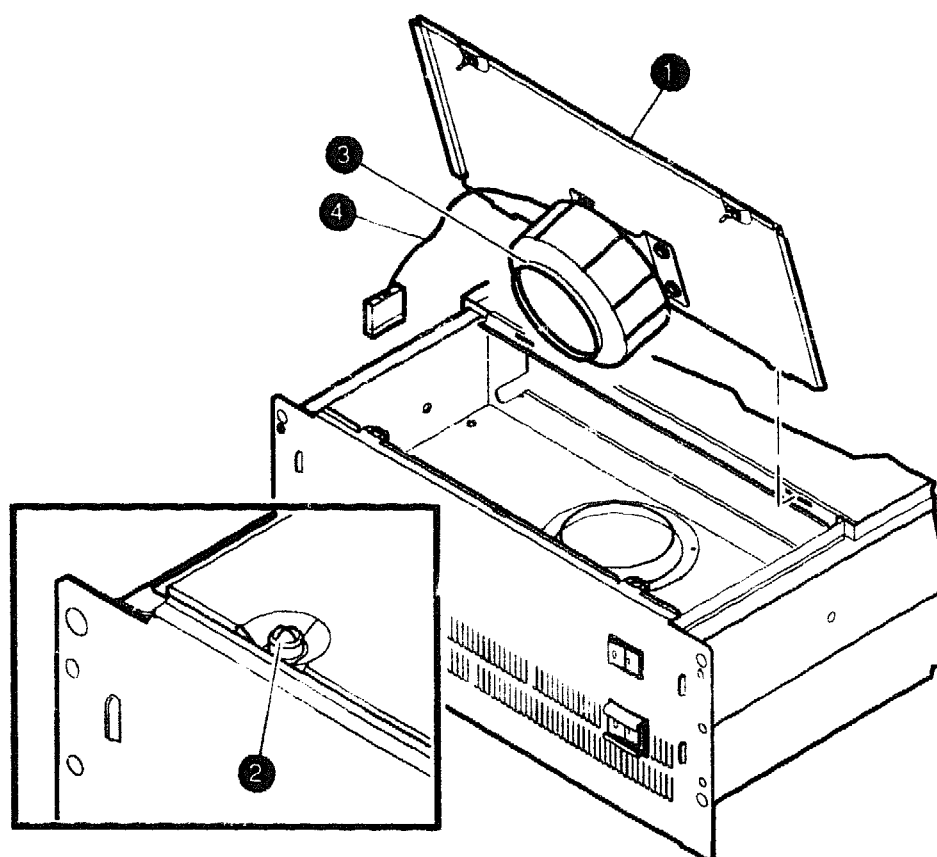
Figure 3-8 Opening the CPU Drawer Front Top Cover
