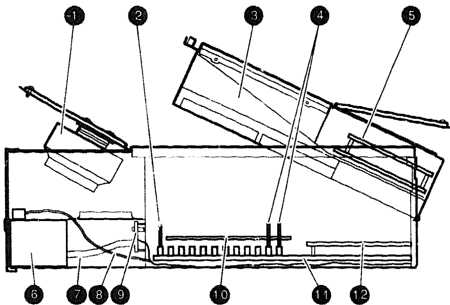
Figure 1-8 CPU Drawer
