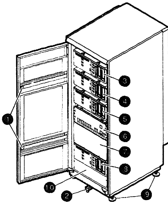
Figure 1-2 The DECsystem 5900 System—Front Open-Door View
