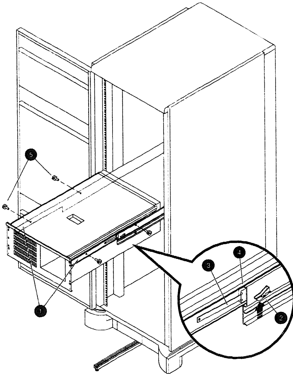
Figure 4-77 Installing a Mass Storage Drawer 2
