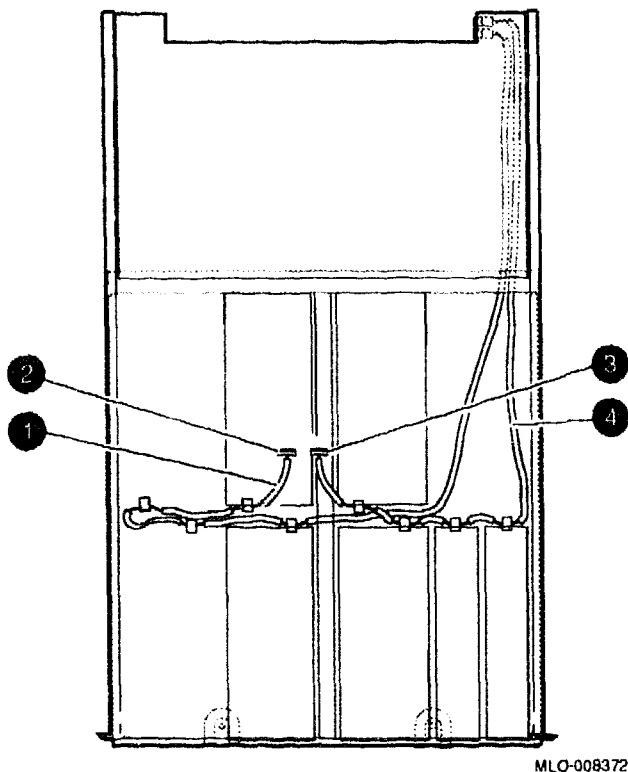
Figure 4–30 Split Bus Configuration for Mass Storage Drawer 1
