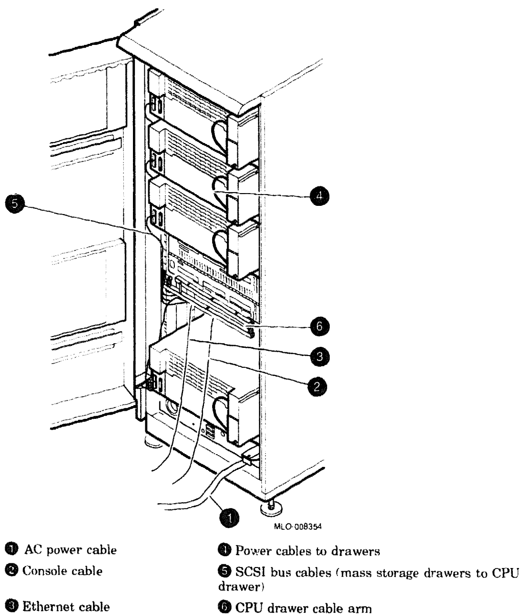
Figure 1-5 Sample Power Cable/Bus Configuration
