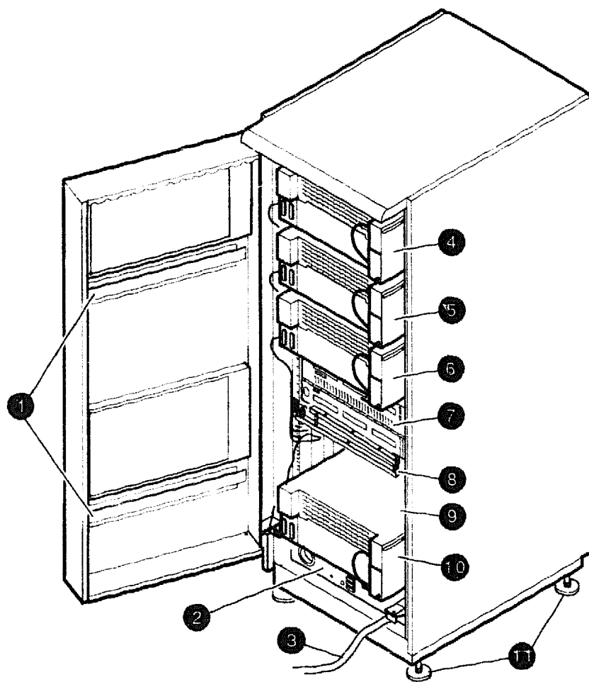
Figure 1-3 The DECsystem 5900 System—Rear Open-Door View
