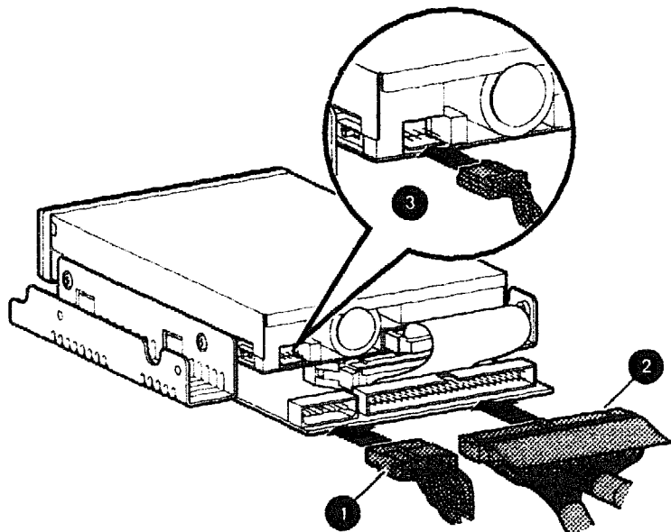
Figure 4-39 Disconnecting/Connecting an RX26
