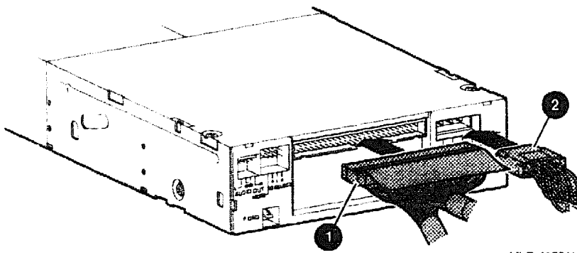
Figure 4-37 Disconnecting/Connecting an RRD42
