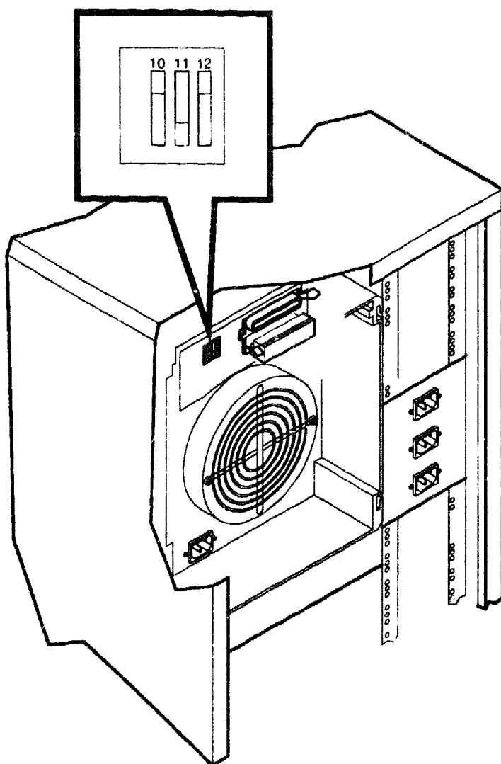
Figure 4-66 SCSI ID Switches on a TZ857
