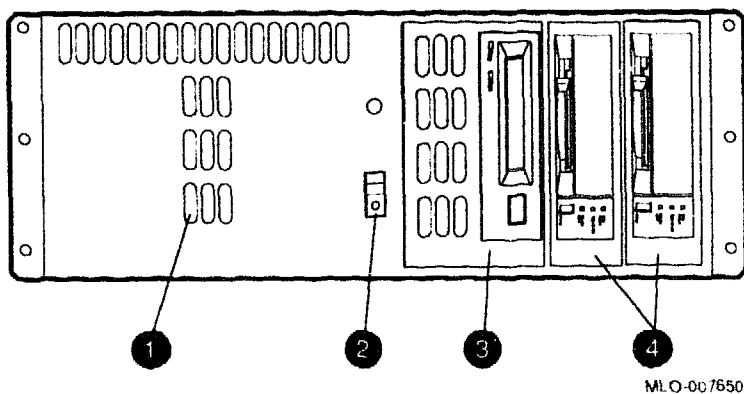
Figure 1-13 Mass Storage Drawer 1 Front Panel
