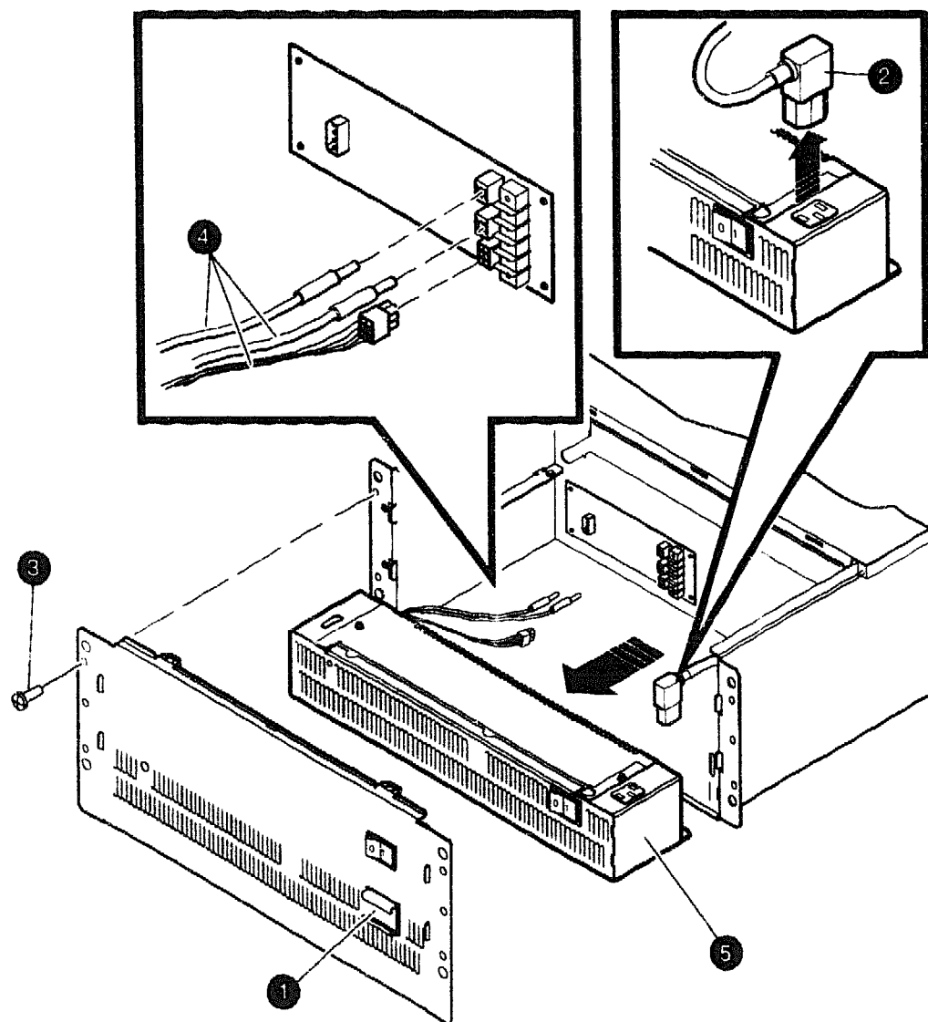
Figure 3-13 Removing the CPU Drawer Power Supply
