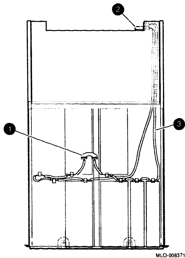
Figure 4-28 Single Bus Configuration for Mass Storage Drawer 1
