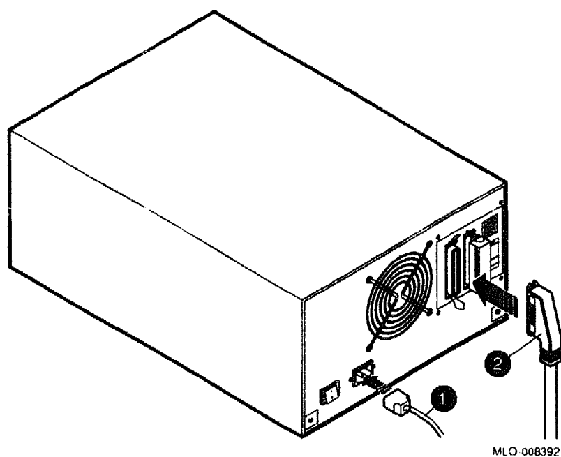
Figure 4-63 Disconnecting/Connecting an External TZ85
