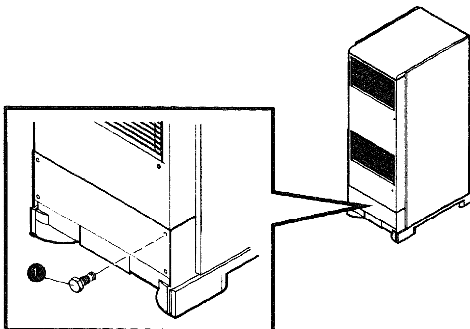
Figure 2-6 Attaching the Lower Rear Skirt Panel
